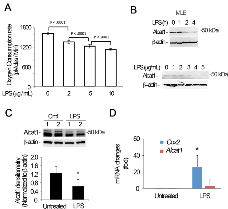
Fig. 1. LPS triggers Alcat1 degradation. (A–C) MLE cells were treated with LPS at varying concentrations (B, lower panels) or times (B, upper panel; fixed LPS concentration of 4 µg/ml). The oxygen consumption rate of cells was analyzed with a seahorse XF analyzer (A), or cell lysates were immunoblotted for Alcat1 and β-actin (B). (C) C57BL6 mice were treated with LPS (5 mg/kg) intratracheally overnight, and whole-lung tissue lysates were analyzed by immunoblotting for Alcat1 and β-actin. (D) Total cellular RNA was isolated from untreated or LPS-treated MLE cells in B (4 µg/ml for 16 h), and quantitative PCR analysis was conducted to determine steady-state mRNA levels using Alcat1 -specific primers. Cox2 was used as a positive control. * P <0.05, Cox2 mRNA changes in untreated versus LPS-treated cells (Student's t -test). Data in each panel represents n =3 separate experiments. Means±s.e.m. are shown.
