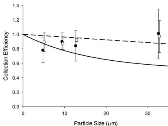
Figure 4. Comparison of sampler collection efficiency of the new sampler at 2 L/min (•) vs 10 L/min (○) flow rates. Data points are slightly offset to enable comparison of error bars, which represent one standard deviation. The data are compared against the inhalable particulate matter (IPM) criterion (solid line) and the low-velocity inhalability Curve (dashed line).
