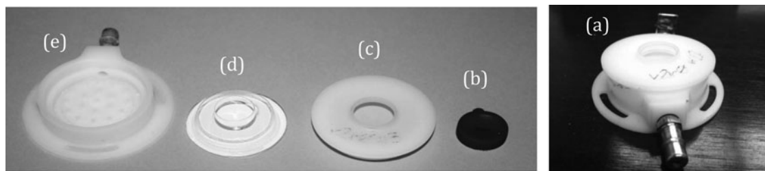
Figure 1. The newly designed sampler, disassembled: (a) housing, (b) capsule and filter, (c) inlet, and (d) inlet cover. To assemble: capsule/filter is placed in housing, then inlet placed on top, followed by the inlet cover (e). Photo courtesy of Tracy M. Rees.
