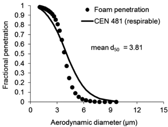
(b) 3 h sampling at 1 \text{ l min}^{-1} in a relative humidity of 95 %
