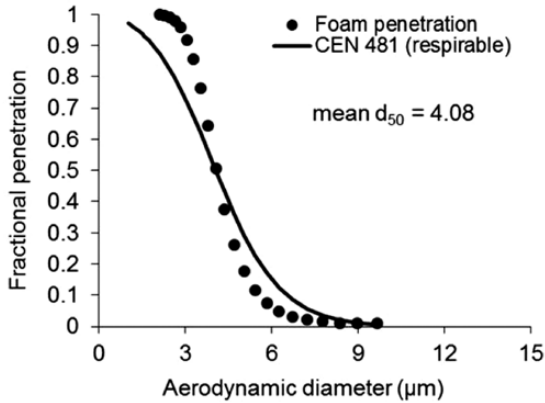
(a) At 1 \text{ l min}^{-1} and relative humidity 47 %
