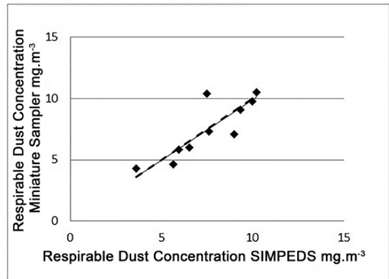
Figure 8 Comparison of respirable dust concentrations between the miniature sampler at 0.8 l min -1 and SIMPEDS samplers when exposed to aerosols from the cutting of sandstone using a Mitre saw.
