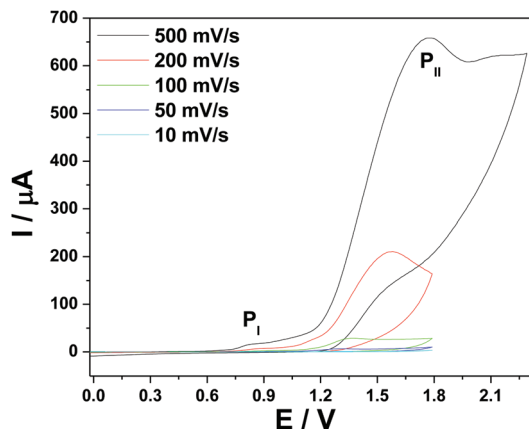
Fig. 3 CV of 0.1% v/v 2,4-TDI in [C_4mpy][NTf_2] with varying of scan rates. Glassy carbon, silver and platinum electrodes were used as the working, reference and counter electrodes, respectively. All potentials were calibrated based on the Fc/Fc^+ redox couple. Air was the background gas for all these measurements. All curves presented herein are taken from the first cycle of the CV measurements.
