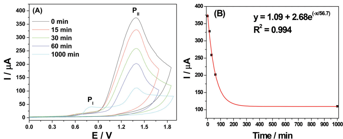
Fig. 4 (A) CV of 2,4-TDI oxidation process in [C_4mpy][NTf_2] in an air environment, on a glassy carbon electrode. The concentration of 2,4-TDI was 10\text{ }\mu\text{L} in 1\text{ mL} ionic liquid (1.0% v/v). Silver and platinum wires were the reference and counter electrodes, respectively. Measurements were performed with different time intervals after the three-electrode system had been setup. The scan rate was 100\text{ mV s}^{-1} . All potentials were calibrated based on the Fc/Fc^+ redox couple. All curves presented herein are taken from the first cycle of CV measurements. (B) The corresponding calibration curve. Air was the background gas for all these measurements.
