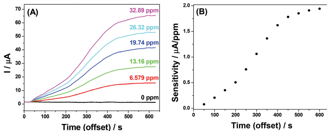
Fig. 9 (A) Real time chronoamperometry detection of gas phase 2,4-TDI in [C_4mpy][NTf_2] . Sensing potential was set constant at 1.4 V. Glassy carbon, silver and platinum electrodes were used as the working, reference and counter electrodes, respectively. Air was the background gas. Data sampling rate is 0.2 second per data point. (B) Plot of the selected sensitivity values at different time scales.
