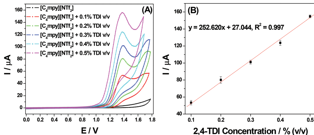
Fig. 8 (A) CV sensing of liquid phase 2,4-TDI in [C_4mpy][NTf_2] on a glassy carbon electrode, in air. Concentration of 2,4-TDI varied from 0.1% v/v to 0.5% v/v. Silver and platinum electrodes were used as the reference and counter electrodes, respectively. The scan rate was 100\text{ mV s}^{-1} . All potentials were calibrated based on the Fc/Fc^+ redox couple. All curves presented here are taken from the first cycle of the CV measurements. (B) Calibration curve of the current vs. 2,4-TDI concentration, with error bars. Air is the background gas.
