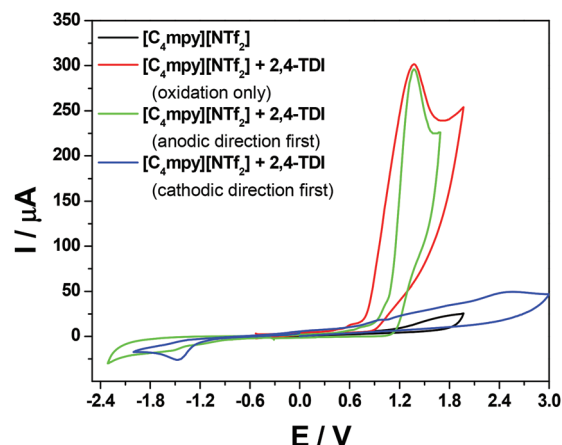
Fig. 2 CV of pure [C_4\text{mpy}][\text{NTf}_2] (black), in the presence of 1.0% v/v 2,4-TDI in the narrow anodic potential window (red), in wider potential window scanning to the anodic potential direction first (green), and in wider potential window scanning to the cathodic potential direction first to form superoxide radical thereby showing no oxidation current for 2,4-TDI (blue). Air was the background gas for all these measurements. All curves presented herein are taken from the first cycle of the CV measurements.
