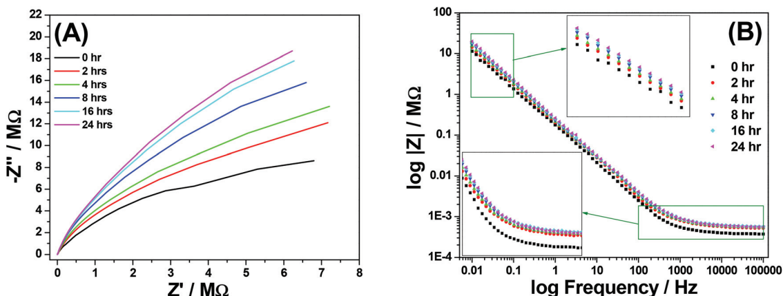
Fig. 5 (A) Nyquist plots measured at various time intervals with 1% v/v 2,4-TDI in [C 4 mpy][NTf 2 ] on a glassy carbon electrode. Silver wire and platinum wire were the reference and counter electrodes, respectively. (B) The Bode plots measured at various time intervals with 1% v/v 2,4-TDI in [C 4 mpy][NTf 2 ] on a glassy carbon electrode. Silver wire and platinum wire were the reference and counter electrodes, respectively. (C) The Bode plots of Z' (the real part of the impedance) changes at different frequencies. (D) The Bode plots of Z'' (the imaginary part of the impedance) changes at different frequencies. The EIS experimental parameters: AC bias was 5 mV, and the DC input was 0 V vs. open circuit. Air is the background gas.
