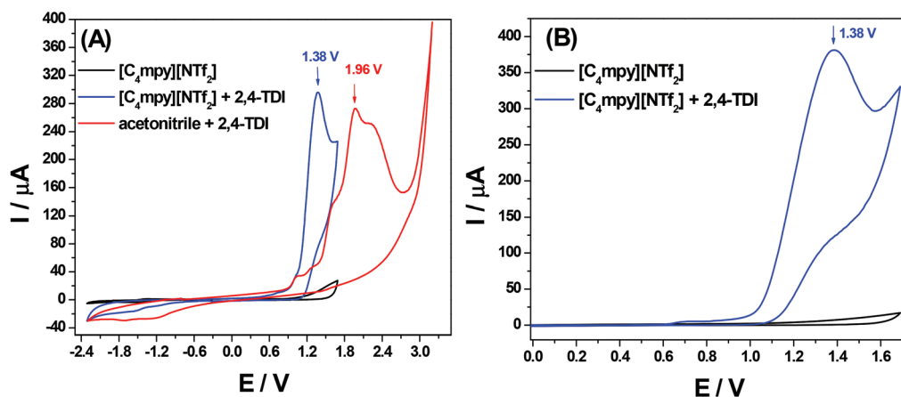
Fig. 1 (A) CV of pure [\text{C}_4\text{mpy}][\text{NTf}_2] (black), 1% v/v 2,4-TDI [\text{C}_4\text{mpy}][\text{NTf}_2] (blue), and 1% v/v 2,4-TDI in acetonitrile with 0.1 M TBAP as a supporting electrolyte (red). The concentration was 1.0% v/v. Glassy carbon, silver and platinum electrodes were used as the working, reference and counter electrodes, respectively. The scan rate was 100 \text{ mV s}^{-1} . All potentials were calibrated based on the \text{Fc}/\text{Fc}^+ redox couple. \text{N}_2 was used as the background gas. CV scanned toward the negative potential direction first. (B) CV for 1 mL of pure [\text{C}_4\text{mpy}][\text{NTf}_2] and in the presence of 1% v/v 2,4-TDI in the potential window of 0 to 1.7 V. All curves presented here are taken from the first cycle of the CV measurements.
