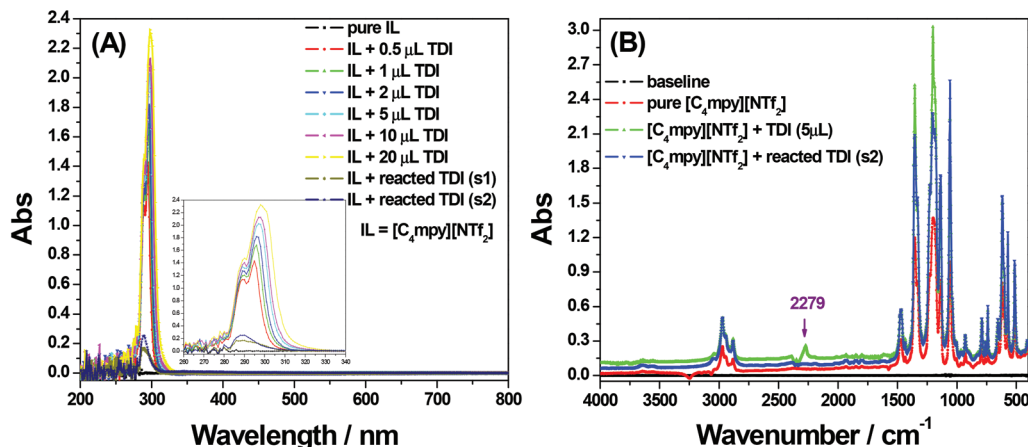
Fig. 6 Spectroscopic characterization of the electrochemical reaction of 2,4-TDI in [C_4mpy][NTf_2] on the glassy carbon surface: (A) UV-Vis method, and (B) FTIR method (transmission mode). 2,4-TDI concentration varied from 0.05% v/v to 2% v/v.
