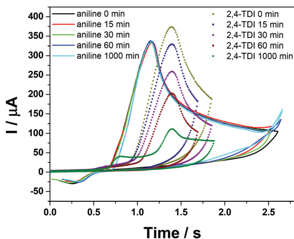
Fig. 7 CV of [C 4 mpy][NTf 2 ] adding 1% v/v aniline (solid lines) and 1% v/v 2,4-TDI (dotted lines), at different testing time intervals, in air. Glassy carbon, silver and platinum electrodes were used as the working, reference and counter electrodes, respectively. Measurements were performed with different time intervals after the three-electrode system had been setup. The scan rate was 100 mV s -1 . All potentials were calibrated based on the Fc/Fc + redox couple. All curves presented here are taken from the first cycle of the CV measurements.
