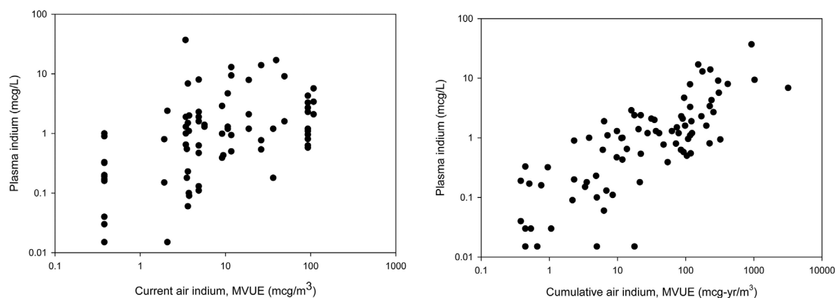
FIGURE 1. Correlation between current (left) and cumulative (right) indium exposure and plasma indium concentration among workers at an indium-tin oxide facility. Current exposure values were assigned on the basis of indium concentrations measured for a participant's current job; cumulative exposure values account for the time a participant spent in each job during employment at the facility. Both air and plasma values plotted using a log scale. The relationship between log transformed plasma indium and log transformed cumulative indium was given by the following equation: \text{Ln}(\text{Plasma Indium}) = -2.35 + 0.662 \cdot \text{Ln}(\text{Cumulative Indium}) , R^2 = 0.60 , P < 0.05 . r_s = Spearman's rank correlation coefficient.
