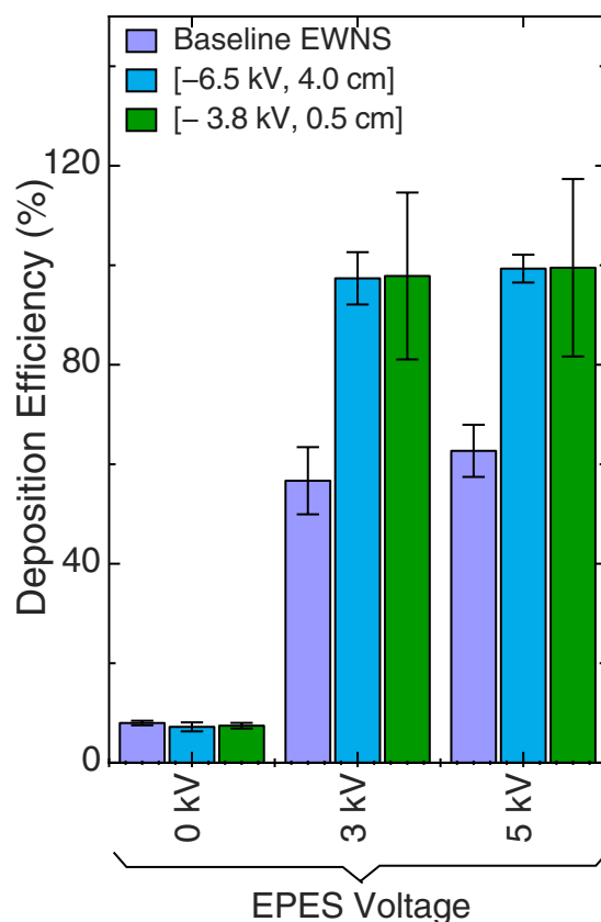
Figure 4. The deposition of the EWNS in the EPES.
