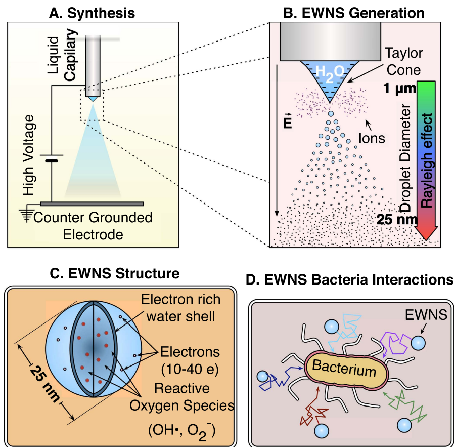
Figure 1. The EWNS synthesis principles. (a) Electrospray occurs when a high voltage is applied between a capillary containing the liquid and the counter electrode. (b) The application of the high voltage results into two distinct phenomena: (i) the electrospray of the water and (ii) generation of reactive oxygen species (ions) that are trapped in the EWNS. (c) The unique structure of EWNS. (d) EWNS due to their nanoscale nature are highly mobile and can interact with airborne pathogens.
