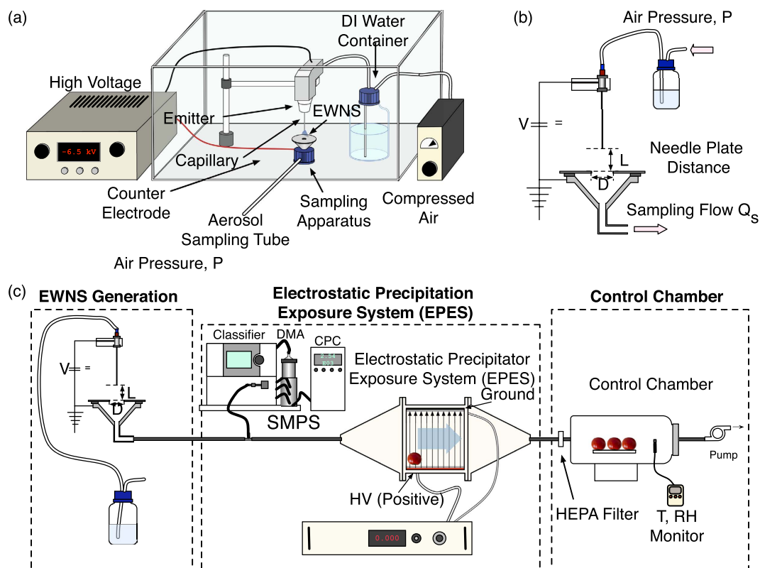
Figure 2. The experimental setup. (a) The Engineered Water Nano-Structures (EWNS) Generation System. (b) Cross section of the sampler and the electrospray device, showing the most important parameters. (c) The experimental setup that was used for the bacteria inactivation.
