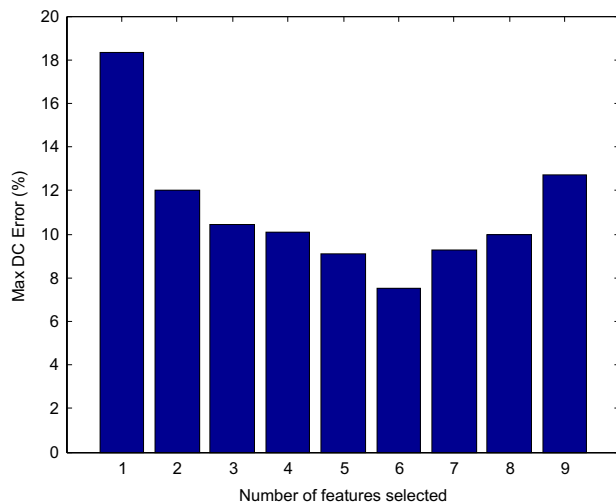
Figure 5. The performance of nine different feature sets based on maximum DC error, \max |\text{ground truth DC} - \text{estimated DC}| .
