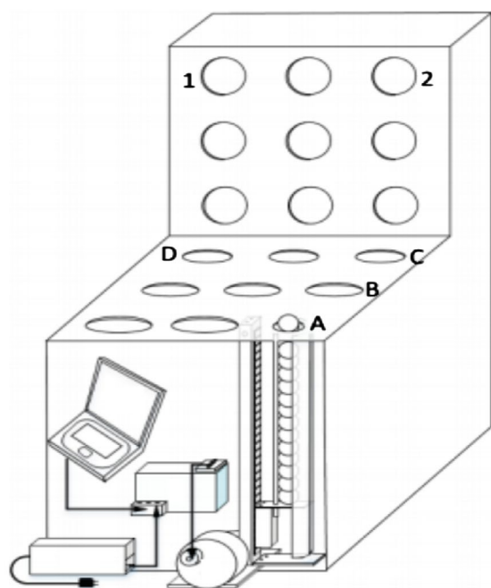
Figure 1. Laboratory task simulation apparatus. The participant grasps a ball from location A and moves it to either locations B, D, 1 or 2, depending on the specified task.
