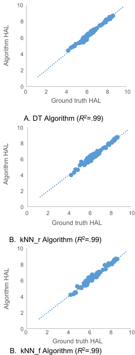
Figure 6. Predicted HAL vs. ground truth HAL for the Decision Tree (DT), k th Nearest Neighbour (41 video training set) (kNN_r), and k th Nearest Neighbour (First cycle training set) (kNN_f) Algorithms, N = 87 .
