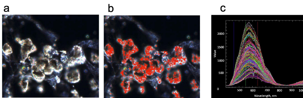
Fig. 9. Hyperspectral images (CytoViva) of the lung tissue of mice at day 7 after pharyngeal aspiration of SWCNTs. The scanned images a) were collected at 40 \times employing an Olympus BX-51 microscope and a 100 W quartz-halogen light source. The pixels that match the SWCNTs spectral profiles were mapped in red b). Spectral data c) was captured with the CytoViva spectrophotometer utilizing an integrated CCD camera.
