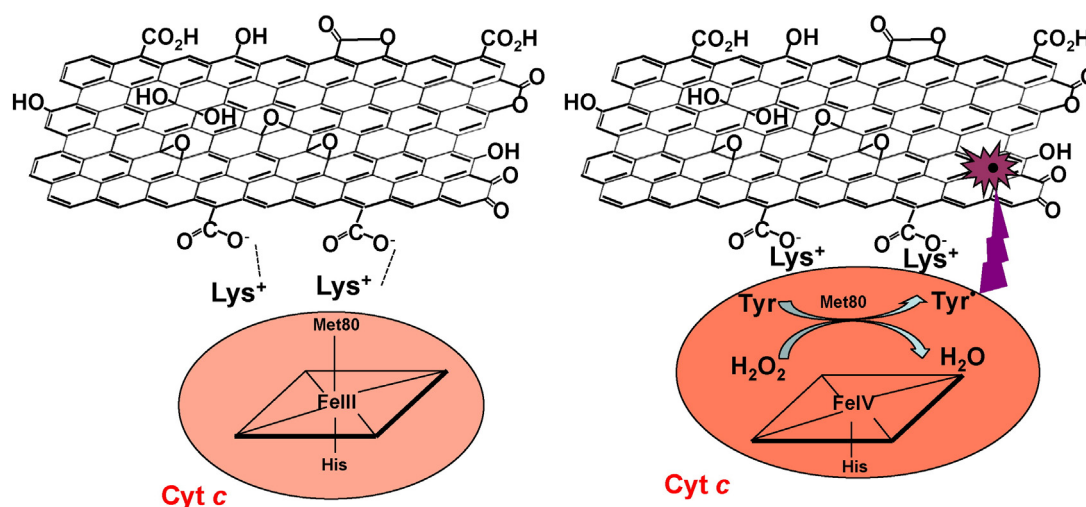
Fig. 3. Cyt c binding and peroxidase activation upon interaction with GO. Eight positive charges on the surface of cyt c (Lys+) can electrostatically interact with the negatively charged oxygen-containing functional groups of GO. This interaction of cyt c with GO leads to protein unfolding associated with the 'awakening' of dormant peroxidase activity. This peroxidase activation of cyt c can trigger – in the presence of oxidizing equivalents ( \text{H}_2\text{O}_2 , organic hydroperoxides) – oxidative modification/degradation of GO.
