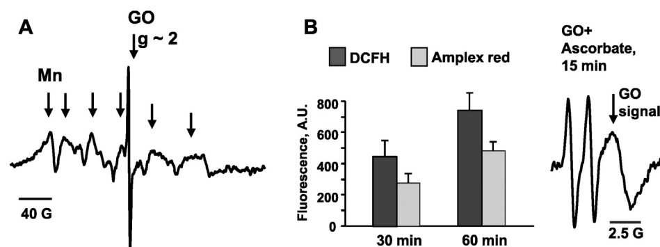
Fig. 1. Paramagnetic properties of GO are accountable for its peroxidase-like activity. A) EPR spectrum of GO measured at 77 K is a composition of a narrow EPR spectrum at g \sim 2.0 which is due to intrinsic paramagnetic properties of GO and hexa-component EPR spectrum of manganese embedded into carbon structure. B) – GO can oxidize peroxidase substrates characterized by low reduction potentials: Amplex red, dichlorofluorescein (DCFH), and ascorbate ( n = 3 ). \text{H}_2\text{O}_2 (100 \mu\text{M} ) was added to the solutions of substrates (50 \mu\text{M} ) and GO (0.1 mg/ml) and formation of fluorescent products was detected at 30 or 60 min. In the absence of GO fluorescence responses from Amplex red or DCFH were lower than 10 A.U. EPR signal of ascorbate (1 mM) could be measured in the absence of \text{H}_2\text{O}_2 but not in the absence of GO (0.5 mg/ml).
