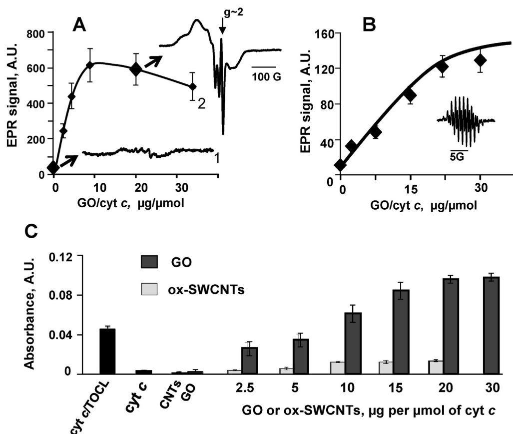
Fig. 5. Binding of GO to cyt c causes unfolding of the protein and increases the accessibility of cyt c active site. A) GO facilitates cyt c nitrosylation as evidenced by low temperature EPR spectroscopy. Magnitude of the signal of nitrosylated cyt c depends on GO/cyt c ratio revealing the increase of the accessibility of cyt c active site towards nitric oxide upon enzyme binding to GO (Vlasova et al., 2006). Insets are EPR spectra of cyt c nitrosylated in the absence (1) and in the presence (2) of GO. EPR spectrum of nitrosylated cyt c/GO complexes includes pronounced narrow GO spectrum at g \sim 2 . Reduced cyt c (100 μM, 500 μM ascorbate) was incubated with GO at 37 °C for 5 min in 50 mM sodium phosphate buffer, pH 7.4, containing 100 μM DTPA, then 750 μM PAPANONOate was added and incubation was continued for additional 15 min. The reaction was stopped by freezing the samples in liquid nitrogen. EPR spectra of nitrosylated cyt c were measured at 77 K. Binding to GO confers peroxidase activity on cyt c: B) Magnitude of EPR spectrum of etoposide-phenoxyl radicals (insert) generated in the peroxidase reaction of cyt c/GO complexes in 2 min after addition of 100 μM H_2O_2 (7.5 μM cyt c) (Kagan et al., 1999); C) Oxidation of peroxidase substrate ABTS by cyt c/GO. Oxidation of ABTS to yield the product with absorbance maximum at 410 nm was performed at reagent concentrations: 5 μM cyt c, 1 mM ABTS and 100 μM H_2O_2 . The effect of GO on cyt c peroxidase activity is compared to the effects of TOCL and ox-SWCNTs.
