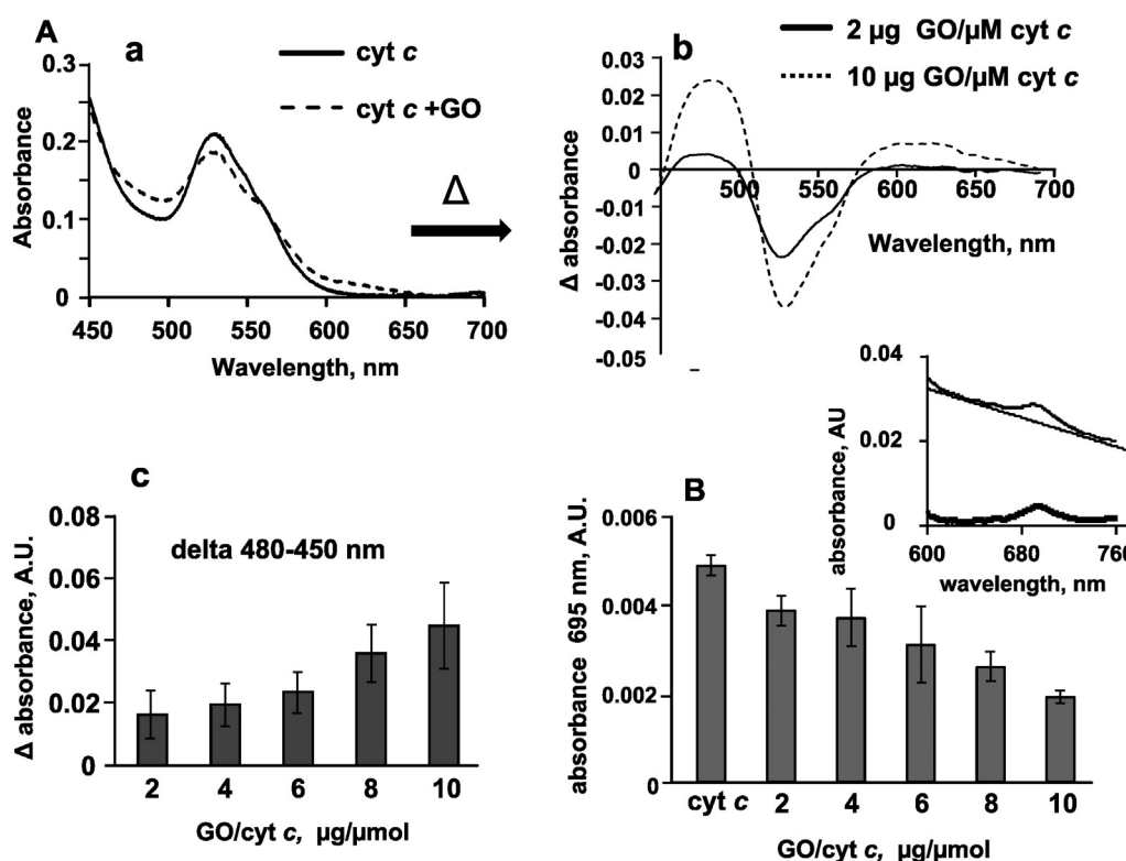
Fig. 4. Absorption spectra of cyt c illustrating GO-induced formation of high-spin form of heme-iron and weakening of the heme iron/Met80 sulfur bond. A) Effect of GO on the formation of high-spin iron state of the hemoprotein. a) Optical absorption spectra of cyt c in the absence (solid line) and in the presence (dashed line) of GO; b) differential absorption spectrum (obtained by subtracting spectrum of cyt c from spectrum of cyt c incubated with GO) shows positive features at 480–495 and 610–625 nm accompanied by a clear trough at 700 nm indicative of high-spin ferric heme; c) Effect of GO on the height of a peak at 480 nm (75 \mu\text{M} cyt c, n = 3 ). B) Dependence of the absorbance of the Fe-S(Met80) bond ( \lambda 695 nm) on GO/cyt c ratio. Characteristic absorbance band at 695 nm is associated with an axial coordination of the heme iron by the sulfur atom of Met80 in cyt c active site. In the presence of GO, loss of absorbance band at 695 nm was observed indicating the disruption or weakening of the Fe-S(Met80) coordination. Inset – optical absorption spectrum of cyt c at region around 695 nm before and after subtracting of baseline. The absorbance was measured in 20 mM HEPES buffer containing 100 \mu\text{M} DTPA (pH 7.4) using 50 \mu\text{M} of cyt c, n = 7-9 .
