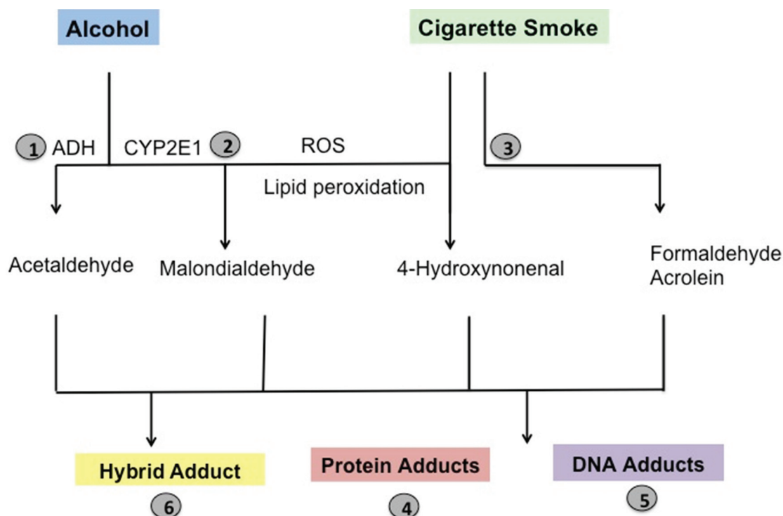
Figure 1. Generation of lung aldehydes and adduct formation. Alcohol is metabolized by alcohol dehydrogenase (ADH) to acetaldehyde (AA). But during chronic alcohol consumption, CYP2E1 is induced leading to generation of ROS like superoxide, hydrogen radical and hydrogen peroxide. This promotes lipid peroxidation and generation of malondialdehyde (MDA) and 4-hydroxynonenal (4-HNE). Cigarette smoke itself contains high concentration of AA, acrolein and formaldehyde. In addition to this, smoking cigarettes also induces local inflammation in lung causing more generation of ROS. This further promotes lipid peroxidation generating more MDA and 4-HNE. Acetaldehyde and MDA could form hybrid adduct through Schiff base reaction when 2 mole of MDA react with 1 mole of AA to form a stable hybrid adduct [74–77].
