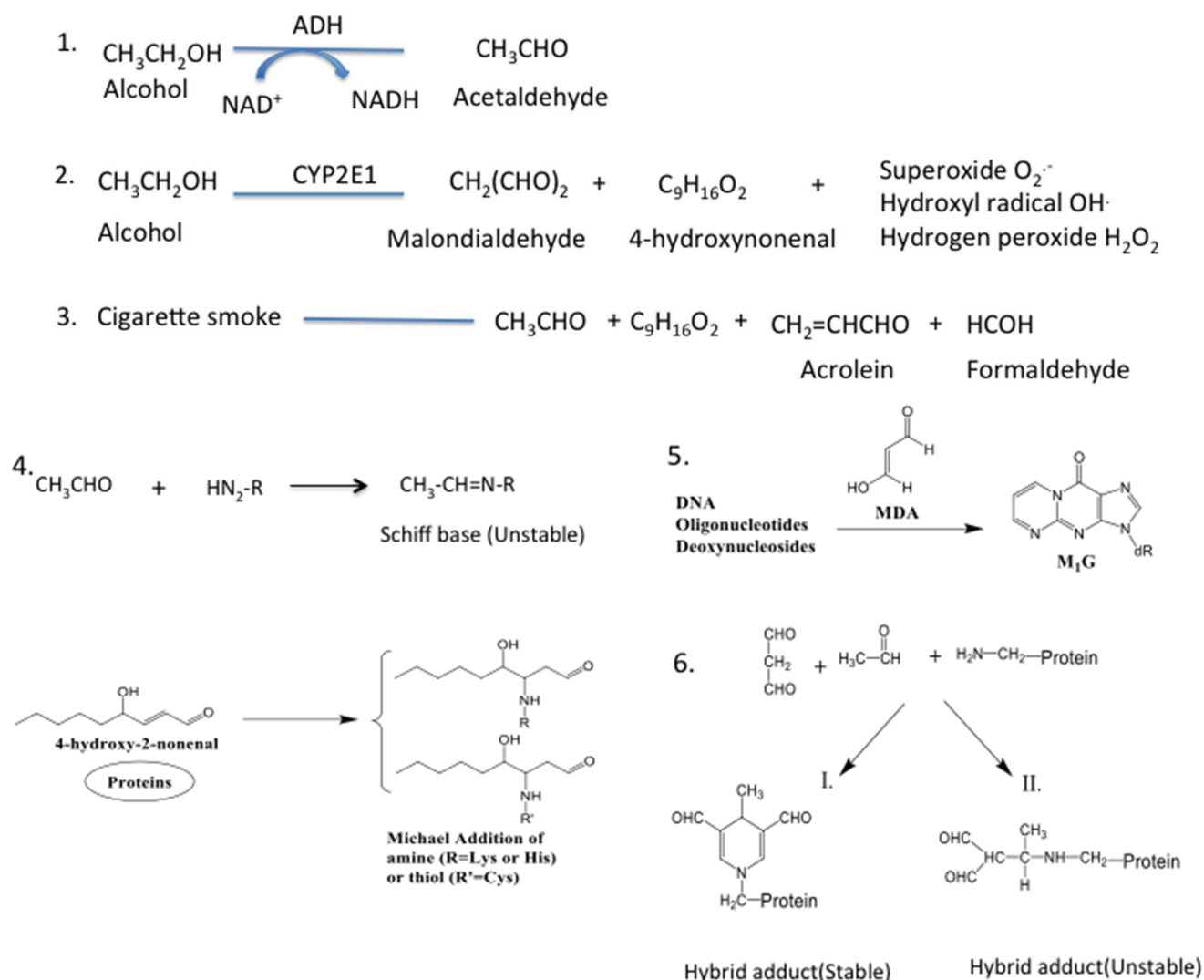
Figure 2. Acetaldehyde and MDA could form hybrid adduct through Schiff base reaction when 2 mole of MDA react with 1 mole of AA to form a stable hybrid adduct. Aldehydes like AA, MDA, acrolein, 4-HNE and formaldehyde could also form protein adduct and DNA adduct. The main reactions involved are Schiff base (involves binding of aldehyde to the alpha group of an N-terminal amino acid of the protein) and Michael addition (involves of binding of aldehyde on amino groups (Lys and His) or thiols (Cys or GSH) [74–77].
