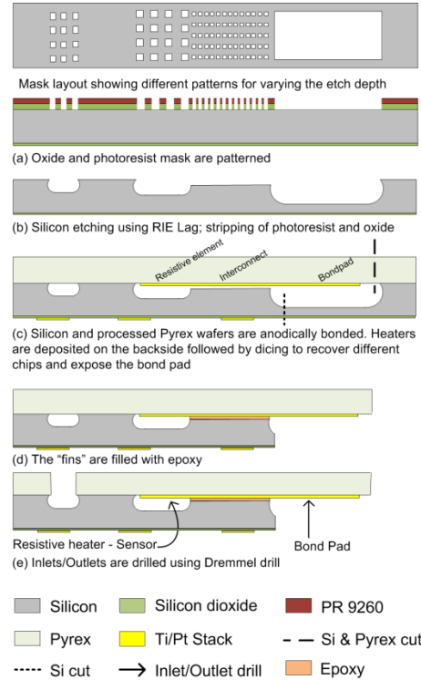
Figure 2-4: Fabrication process (not to scale) shows the silicon etch step in (a) and (b) followed by bonding with the Pyrex wafer with detectors and backside heater/sensor deposition in (c). Finally (d) and (e) show the packaging steps.
