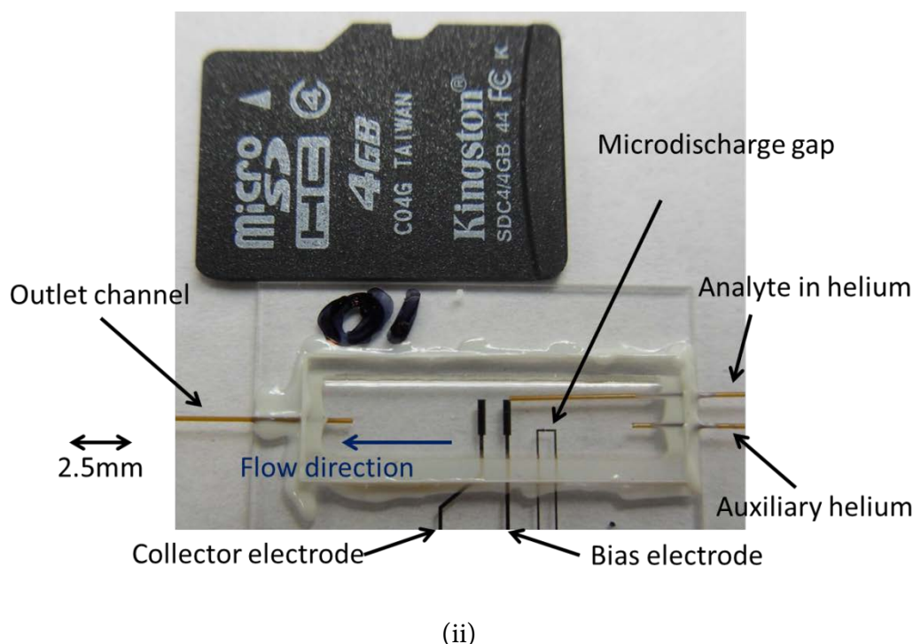
Figure 7-2: (i) Top image shows the fabrication of the detector using Borofloat wafers. The top bottom wafer is patterned in (a), and wet etched and stripped in (b) to obtain the microfluidic channels. In (c) a lift-off on top wafer deposits the patterned metal structures for the electrodes. The wafers are diced and epoxy-bonded in (d). An optical image of the \mu HDID right next to a micro-SDcard is shown at the bottom in (ii).
