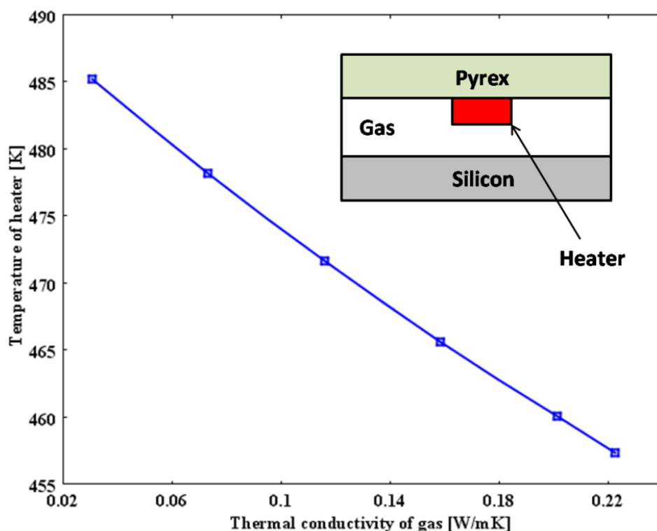
Figure 2-1: A simulated plot of the temperature of a resistive heater in contact with Pyrex on one side and separated from silicon on the other by a gas. A representation of the 2D model with heater used for the simulation is shown in the inset, top right.
