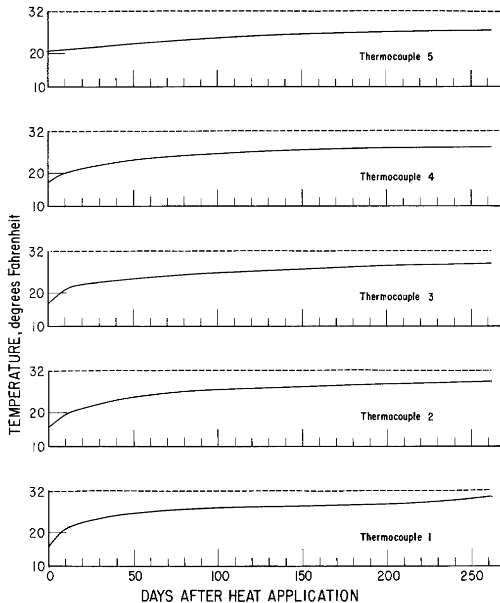
FIGURE 18. - Thermocouple Readings, Back of Silt Room.
