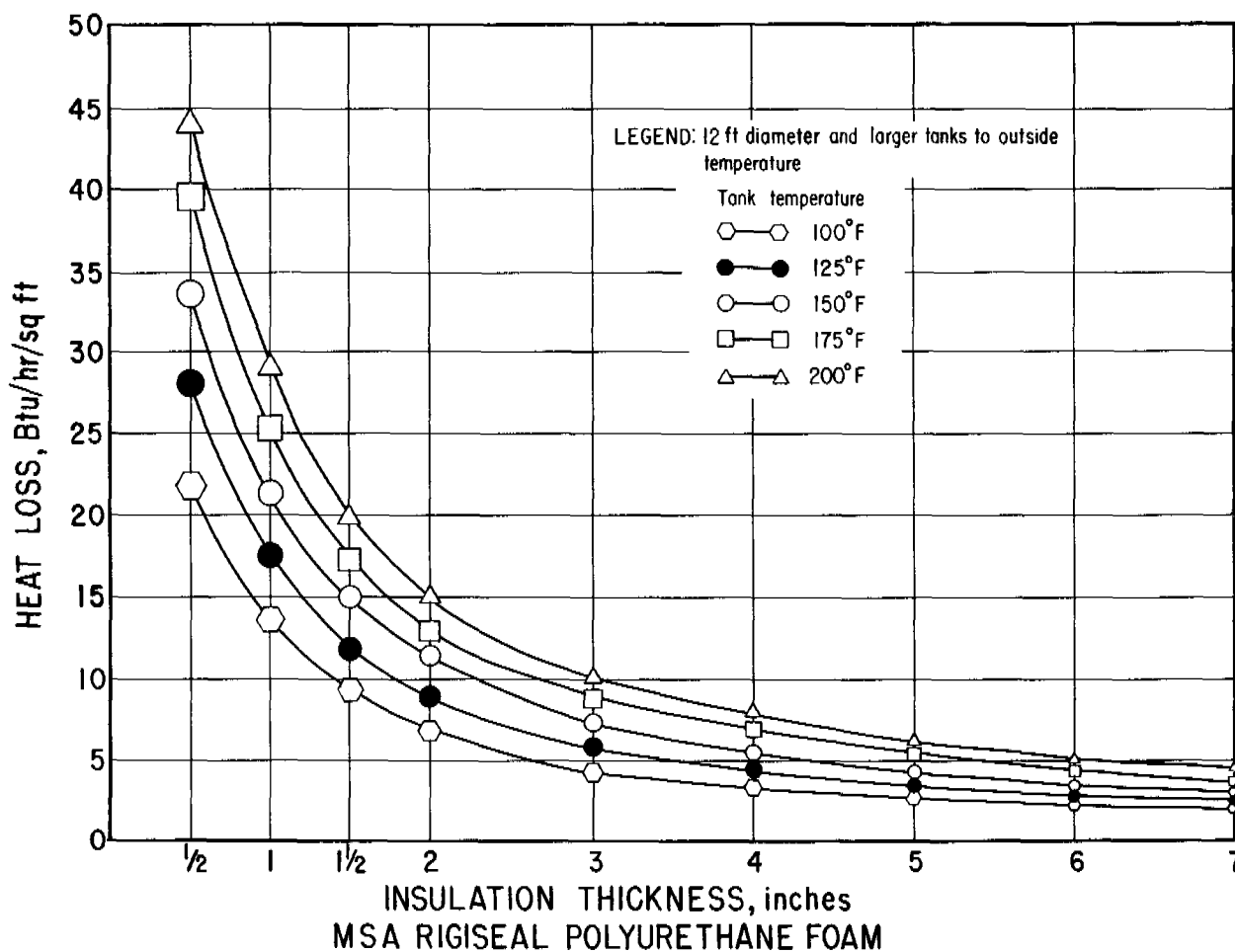
FIGURE 15. - Effect of Insulation Thickness on Heat Loss.
