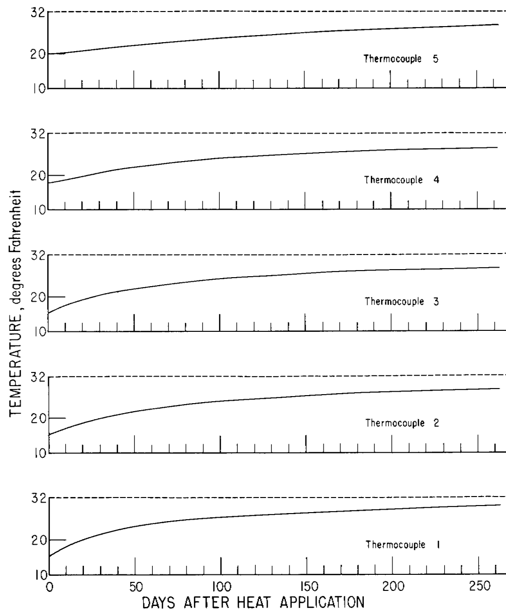
FIGURE 20. - Thermocouple Readings, Side Wall of Silt Room.
