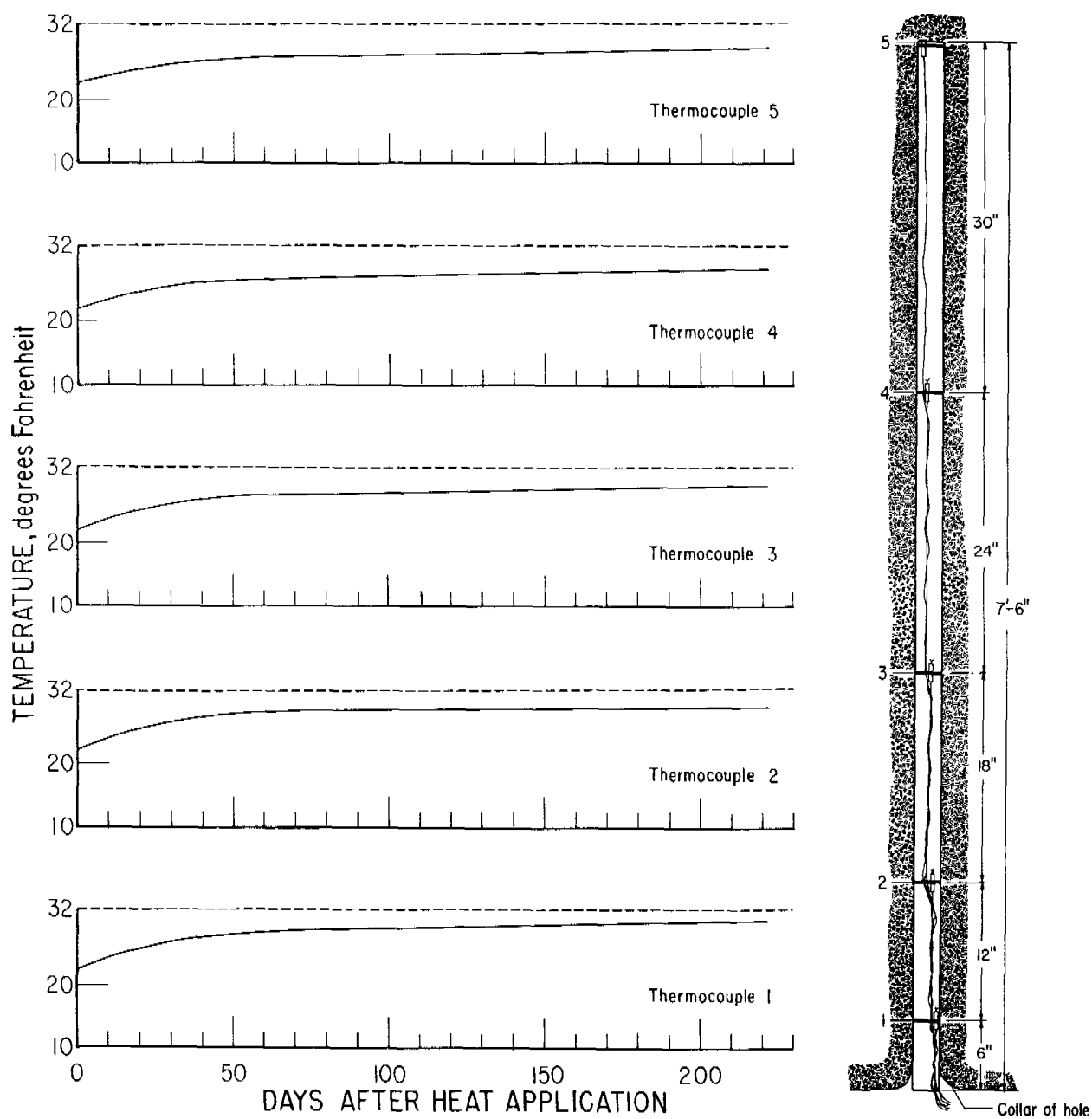
FIGURE 25. - Thermocouple Readings, Side Wall of Gravel Room.
