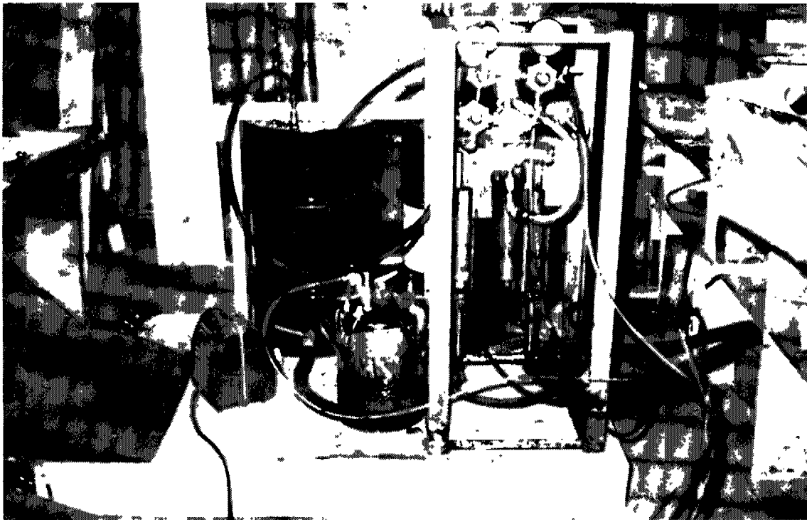
FIGURE 2. - Rigiseal System. B , On sled at Fox, Alaska, installation.
