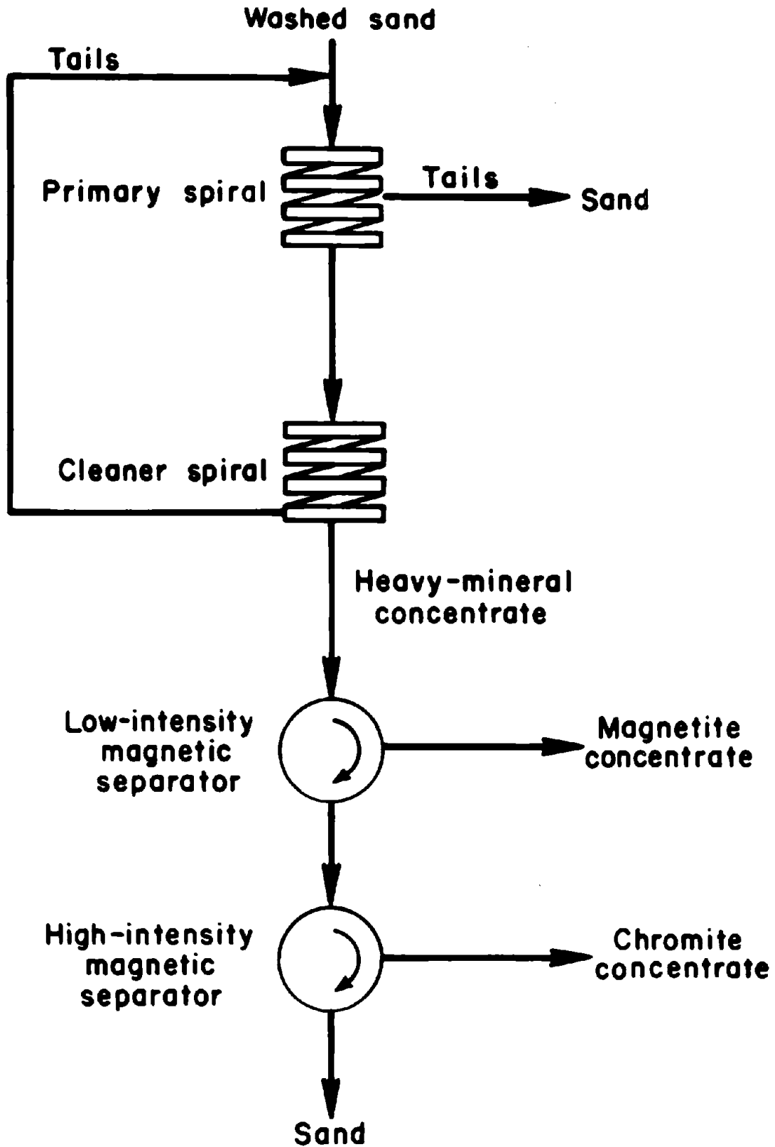
FIGURE 3. - Processing sequence for San Simeon Creek sand.
