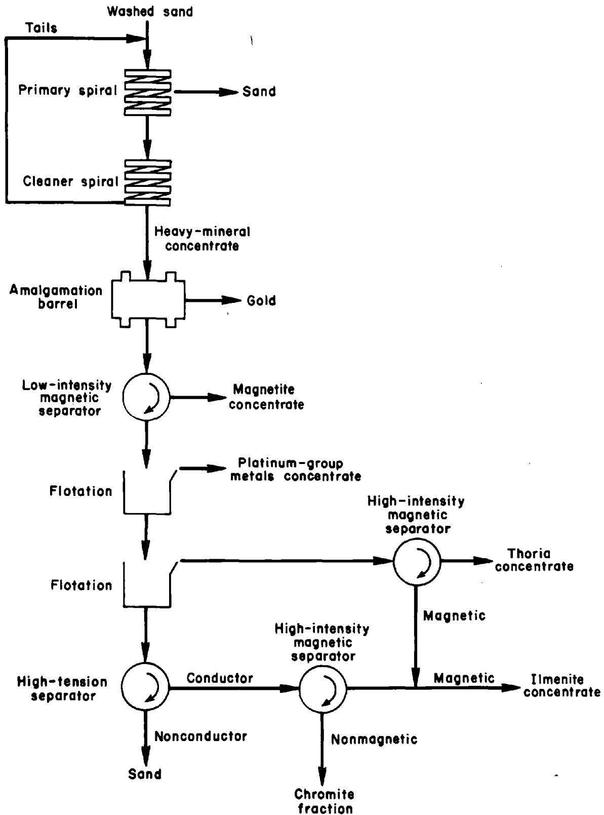
FIGURE 4. - Processing sequence for Merced and San Joaquin Rivers sand.
