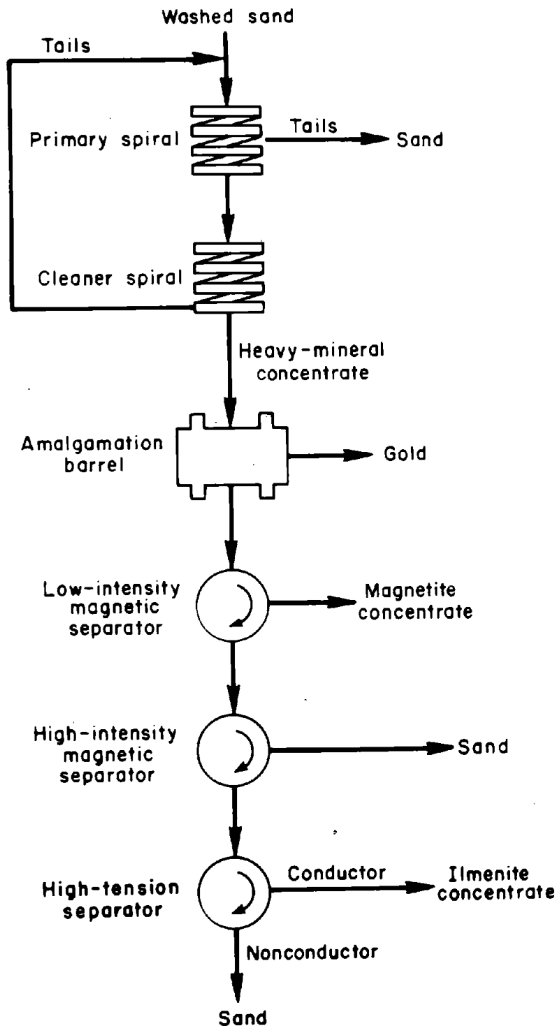
FIGURE 5. - Processing sequence for Big Tujunga, San Gabriel, Otay, and Sweetwater Rivers sand samples.
