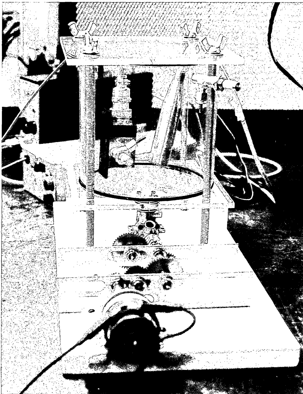
FIGURE 14. - Piston chamberphone.
