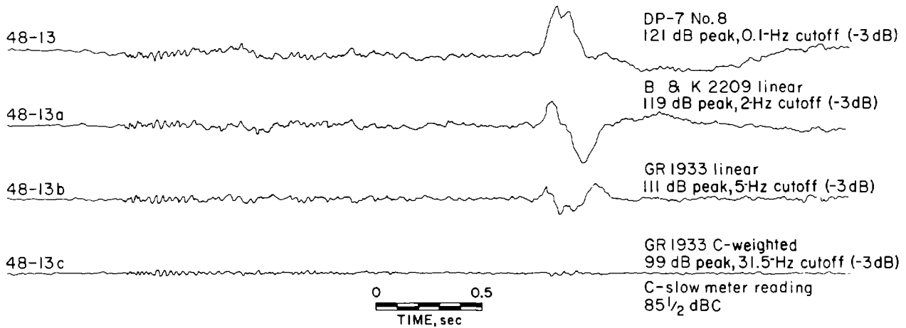
FIGURE 22. - Type II airblast measured four different ways.
