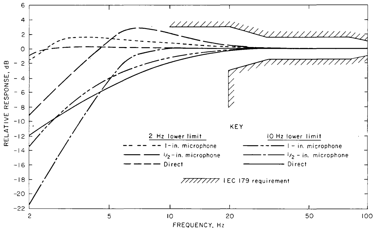
FIGURE 9. - Typical response of SLM input electronics (5).
