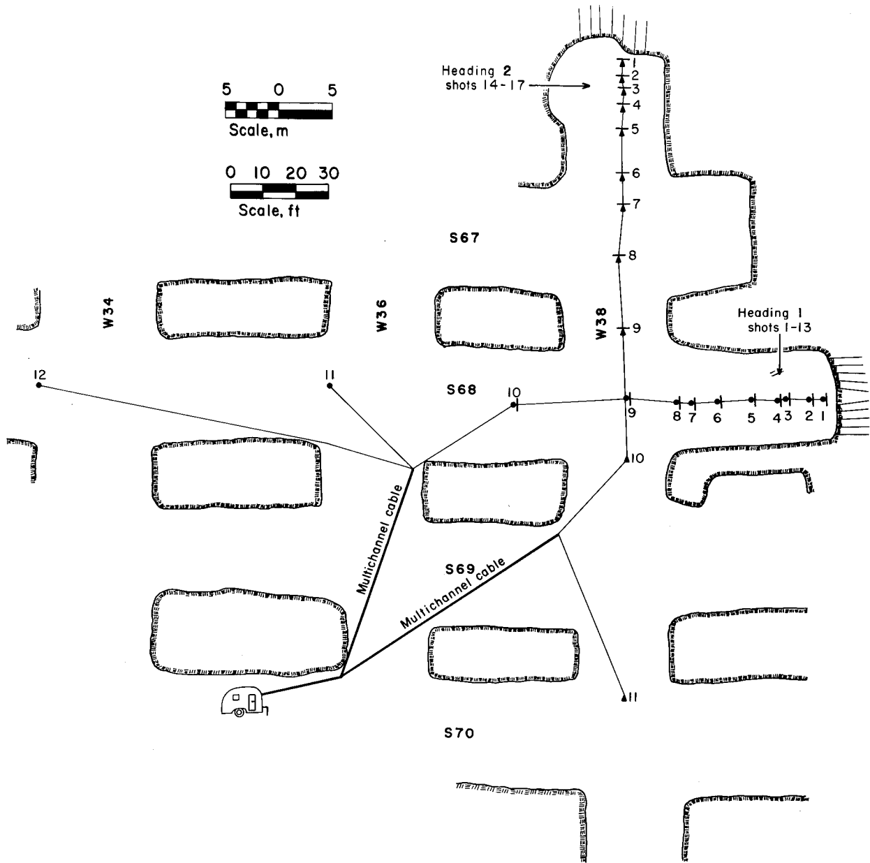
FIGURE 4. - White Pine test headings 1-2.
