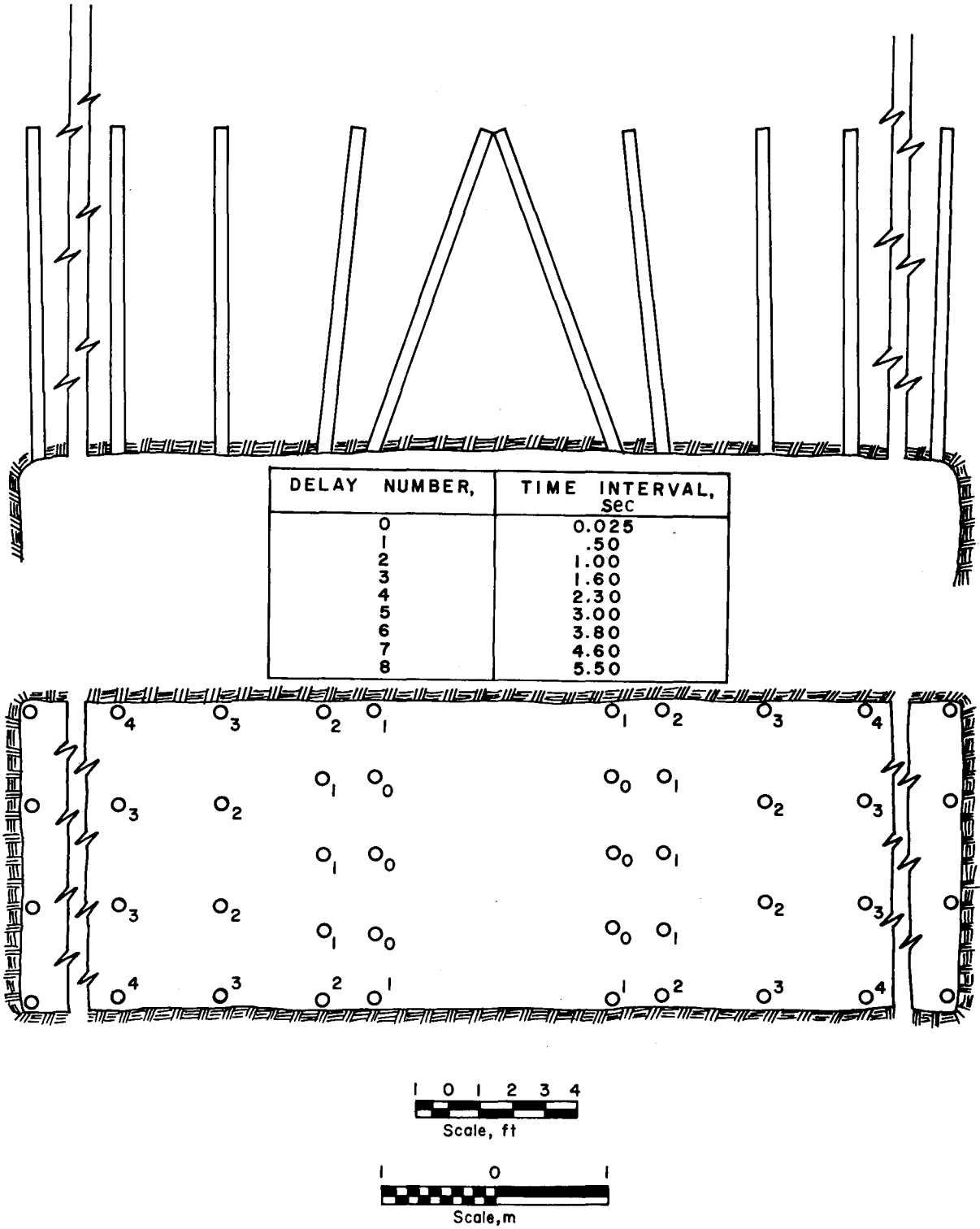
FIGURE 10. - Typical Shullsburg production round.
