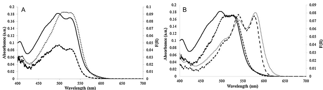
Fig. 3. (A) Comparison of monocyanocobinamide solution spectra and diffuse reflectance spectra on cellulose and glass fiber filter paper. The Kubelka–Munk function is plotted for the diffuse reflectance spectra. Solution spectra for 20 \mu\text{M} \text{CN}(\text{H}_2\text{O})\text{Cbi} (solid line); diffuse reflectance on cellulose filter paper (dashed line) and diffuse reflectance spectra on glass fiber filter paper (dotted line). (B) Comparison of monocyanocobinamide solution spectra and diffuse reflectance spectra on glass fiber paper. Solution spectra for 20 \mu\text{M} \text{CN}(\text{H}_2\text{O})\text{Cbi} in solution before excess KCN is added (solid line) and after KCN is added (dotted line). Diffuse reflectance spectra for \text{CN}(\text{H}_2\text{O})\text{Cbi} on glass fiber paper before excess HCN gas is introduced (short dashed line) and after HCN exposure (long dashed line).
