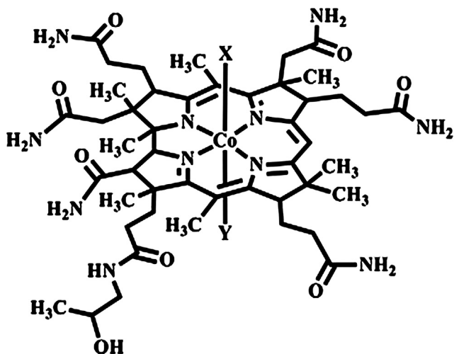
Fig. 1. Structure of cobinamide (Cbi).
