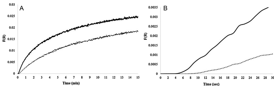
Fig. 5. (A) \text{CN}(\text{H}_2\text{O})\text{Cbi} on glass fiber paper response to 1.0 and 5.0 ppm HCN. 5.0 ppm HCN response at 583 nm (black line), 1.0 ppm HCN response at 583 nm (dotted line). (B) Expanded version of the initial response (in s) to 5.0 ppm HCN at 583 nm (solid line) and 1.0 ppm HCN at 583 nm (dotted line).
