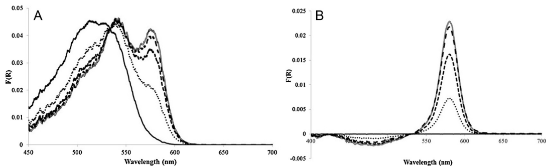
Fig. 4. (A) Monocyanocobinamide response to 5.0 ppm HCN exposure on glass fiber filter paper as a function of time of exposure. \text{CN}(\text{H}_2\text{O})\text{Cbi} before HCN (solid line), 1 min of exposure (dotted line), 5 min of exposure (short dashed line), 10 min exposure (long dashed line) and 15 min exposure (hollow line). (B) Diffuse reflectance spectra when the reflectance spectrum of \text{CN}(\text{H}_2\text{O})\text{Cbi} on glass fiber filter paper was designated as the “blank” (solid line), 1 min exposure (dotted line), 5 min exposure (short dashed line), 10 min exposure (long dashed line) and 15 min exposure (hollow line).
