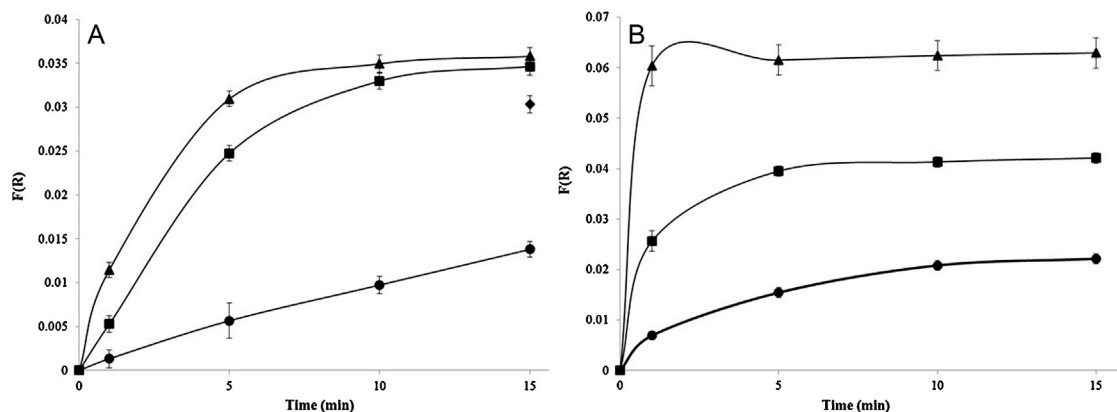
Fig. 6. (A) Average response of \text{CN}(\text{H}_2\text{O})\text{Cbi} on cellulose filter paper to 5 ppm HCN gas as a function of time of exposure at 25%RH (circle), 50%RH (square) and 85%RH (triangle). Error bars are represented by 95% C.I. for n = 3 . (B) Average response of \text{CN}(\text{H}_2\text{O})\text{Cbi} on glass fiber filter paper to 5.0 ppm HCN at various exposure times at 25%RH (circle), 50%RH (square) and 85%RH (triangle). Error bars are represented by 95% C.I. using n = 3 for 50%RH and 85%RH and n = 6 for 25%RH.
