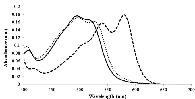
Fig. 2. Spectra of the three cobinamide complexes: \text{OH}(\text{H}_2\text{O})\text{Cbi} (solid line), \text{CN}(\text{H}_2\text{O})\text{Cbi} (dotted line) and (\text{CN}_2)\text{Cbi} (dashed line).
