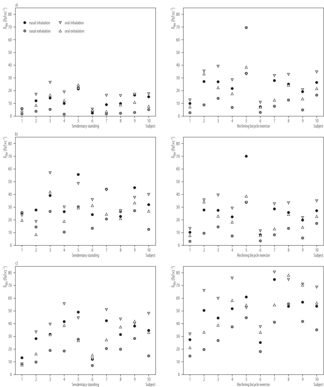
Fig. 1. Mean peak oral and nasal inhalation and exhalation airflow filter resistance of prototype respirators (PR) at sedentary and low-moderate work rates: a) PR3, b) PR6, c) PR9
