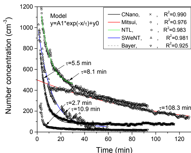
Figure 1. Number concentration as a function of time for different CNT materials. The initial amount of each material tested was 0.2-0.5 g.
