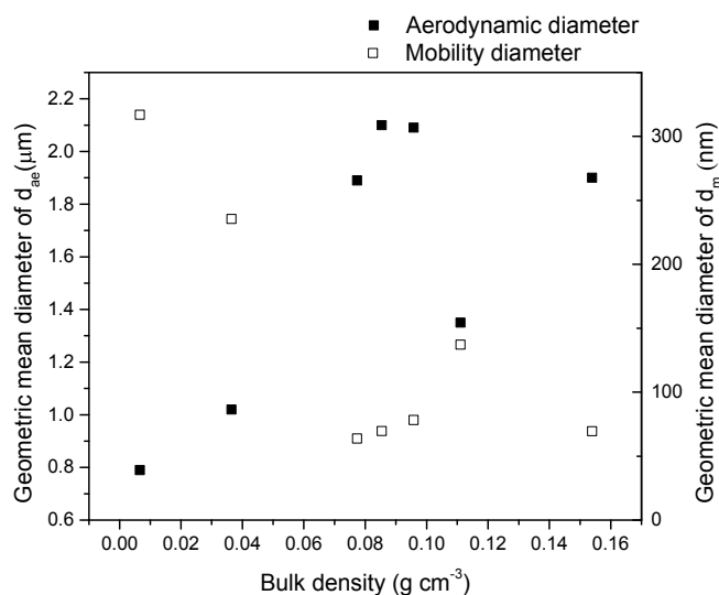
Figure 4. Aerodynamic and mobility diameters as a function of measured bulk density.
