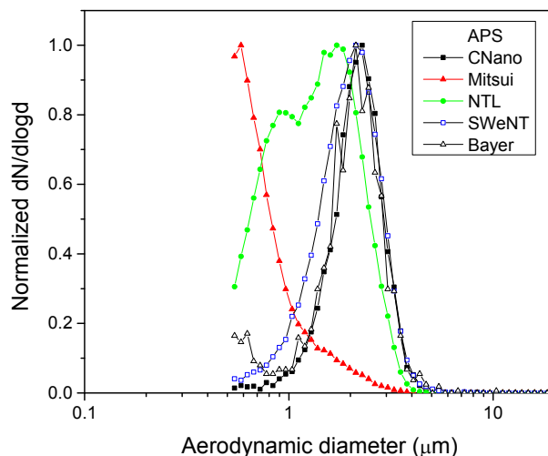
Figure 2. Normalized aerodynamic size distribution of different CNT materials aerosolized by an acoustic generator.
