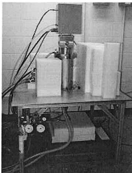
Figure 1. DD neutron generator.
