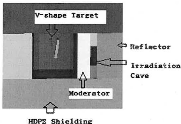
Figure 5. Cross-sectional plot of the NAA system in the MC simulation model.
