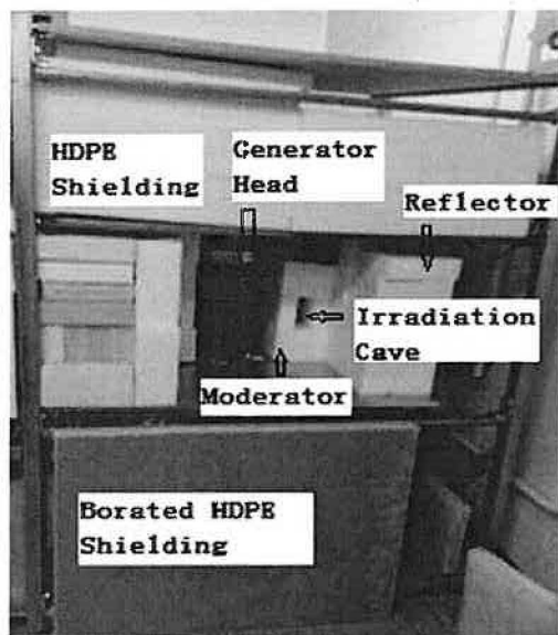
Figure 3. Neutron activation analysis system with moderator/reflector/shielding.
