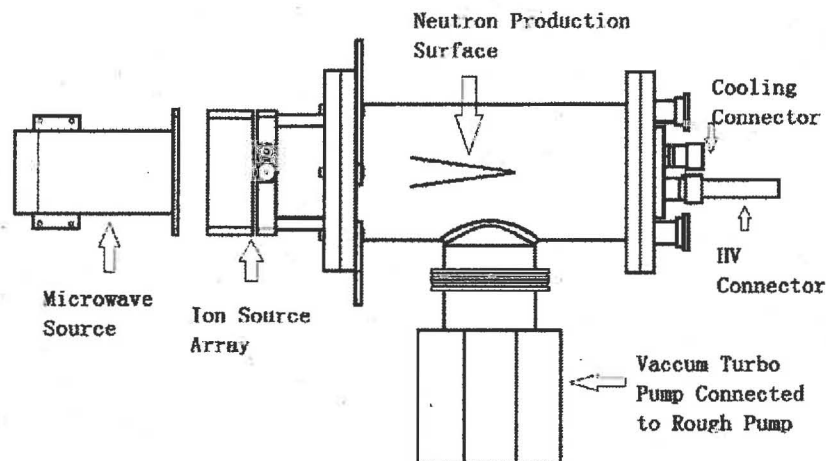
Figure 2. Schematic plot of DD neutron generator head.
