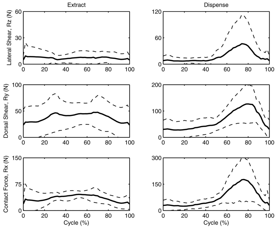
Fig. 7 Variations in the MP joint constraint forces during the extraction and dispensing cycles. The left and right columns of the plots show the forces in the extraction and dispensing phases, respectively. The mean values are shown in solid lines, whereas the standard deviations of the data are shown in dotted lines.
