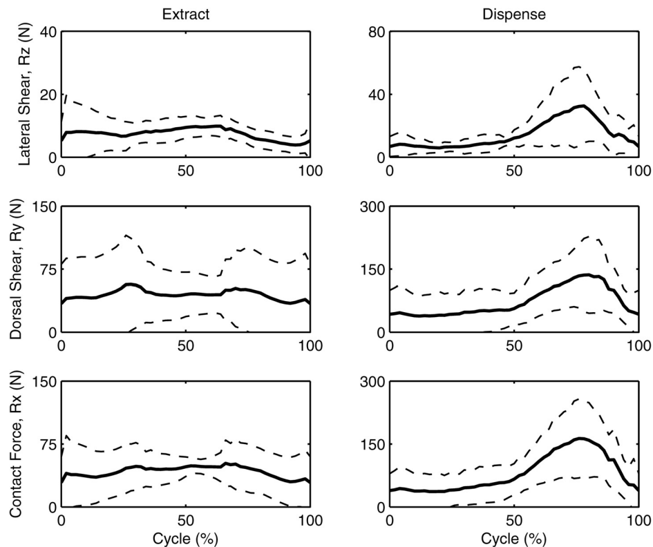
Fig. 6 Variations in the CMC joint constraint forces during the extraction and dispensing cycles. The left and right columns of the plots show the forces in the extraction and dispensing phases, respectively. The mean values are shown in solid lines, whereas the standard deviations of the data are shown in dotted lines.
