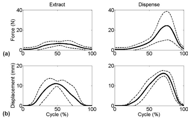
Fig. 5 Histories of the push force and button displacement during the extraction and dispensing cycles. (a) The push force as a function of pipetting cycle. (b) The button displacement as a function of pipetting cycle. The solid lines represent the mean values of all eight subjects' data and the dotted lines are the standard deviations.
