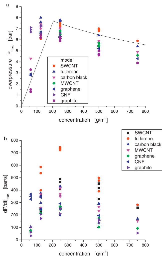
Fig. 2. Concentration dependence of explosion parameters: (a) maximum experimental overpressure, P_{\max} , with thermodynamic curve (solid line) for graphite; (b) maximum dP/dt .
