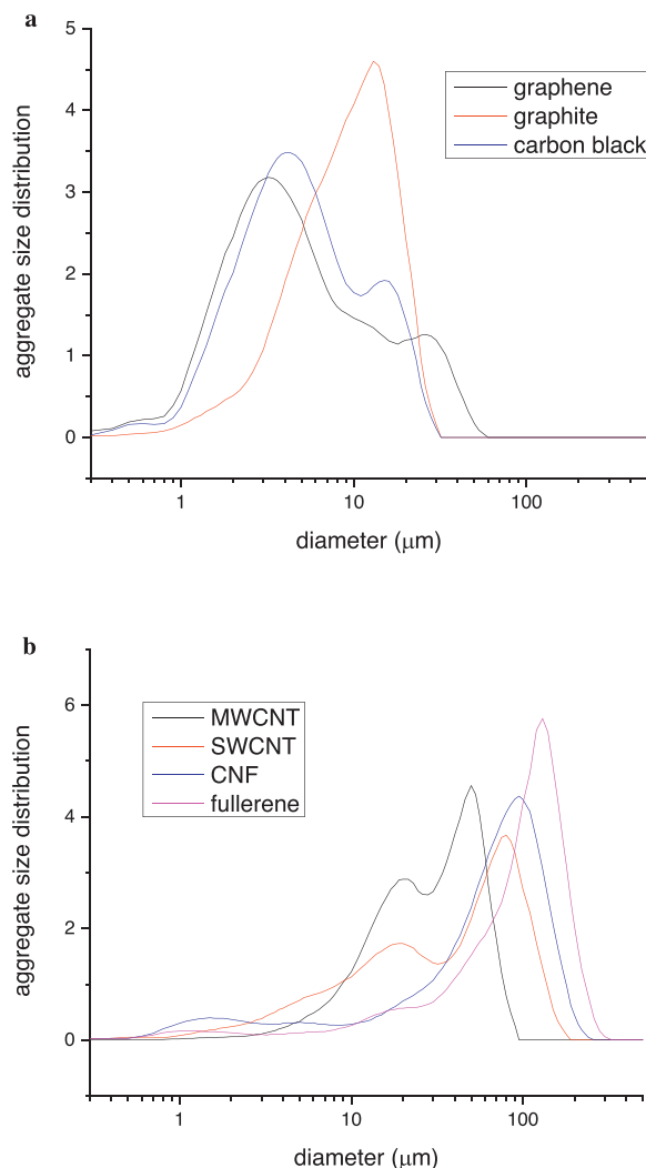
Fig. 1. Aggregate particle size distributions as measured by light scattering: (a) graphene, graphite, carbon black; (b) MWCNT, SWCNT, carbon nanofibers (CNF), fullerene.
