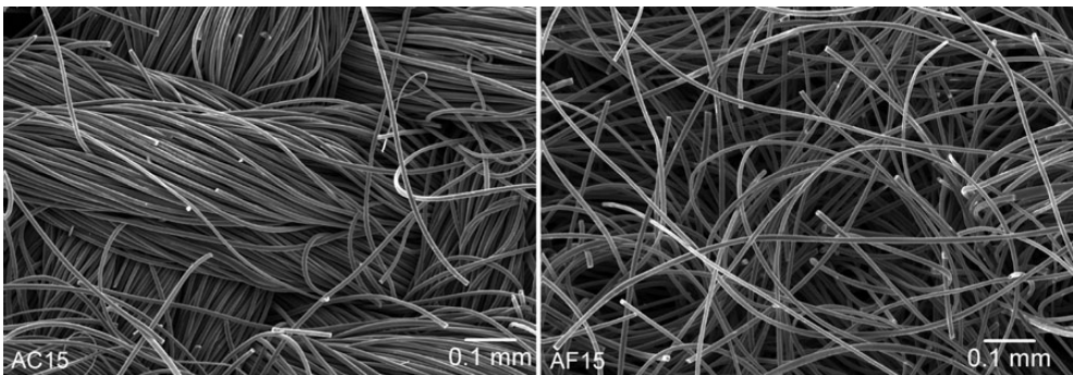
1 SEM images of (a) AC15 and (b) AF15 at ×203 magnifications.
