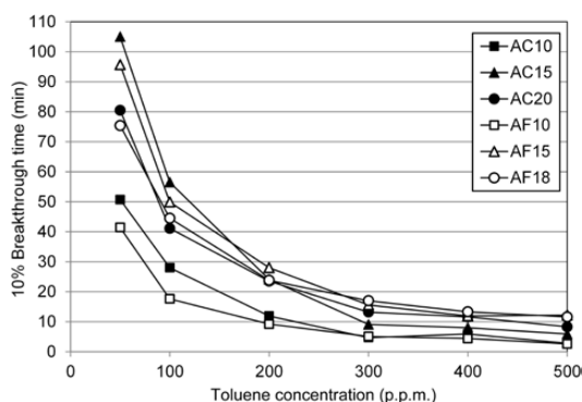
4 10% Breakthrough time as a function of toluene concentration by ACF type at number of ACF layers = 5.
