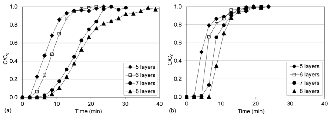
2 Experimental breakthrough curves for (a) AC10 and (b) AF10 by number of layers at C_0 = 500 -p.p.m. toluene.
