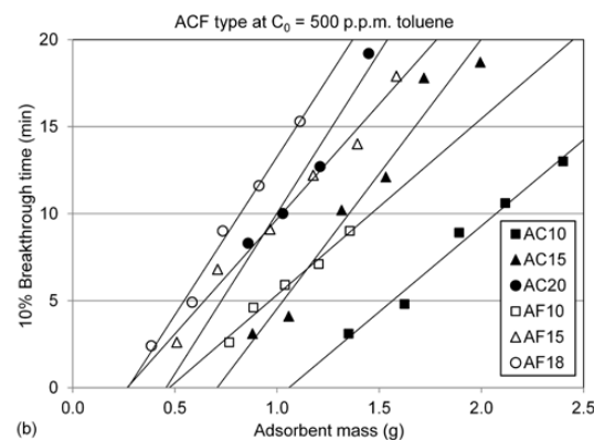
7 10% Breakthrough time of toluene as a function of mass by ACF type at (a) C_0 = 50 p.p.m. and (b) 500 p.p.m.
