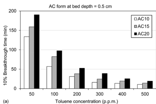
(a) 10% Breakthrough time of toluene by ACF type: (a) AC form and (b) AF form.
