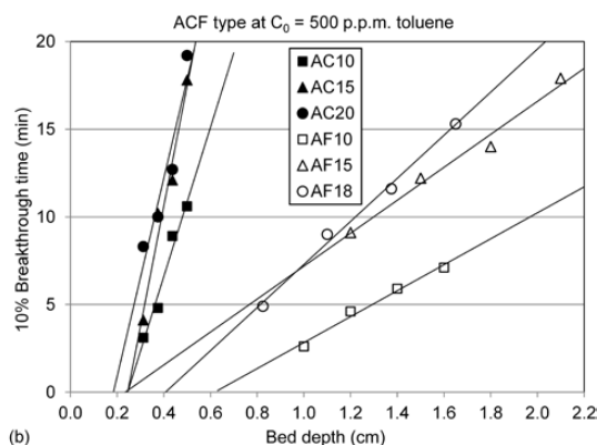
6 10% Breakthrough time of toluene as a function of bed depth by ACF type at (a) C_0 = 50 p.p.m. and (b) 500 p.p.m.
