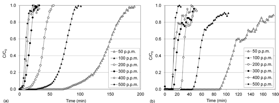
3 Experimental breakthrough curves for (a) AC15 and (b) AF15 by toluene concentration at number of ACF layers = 5.
