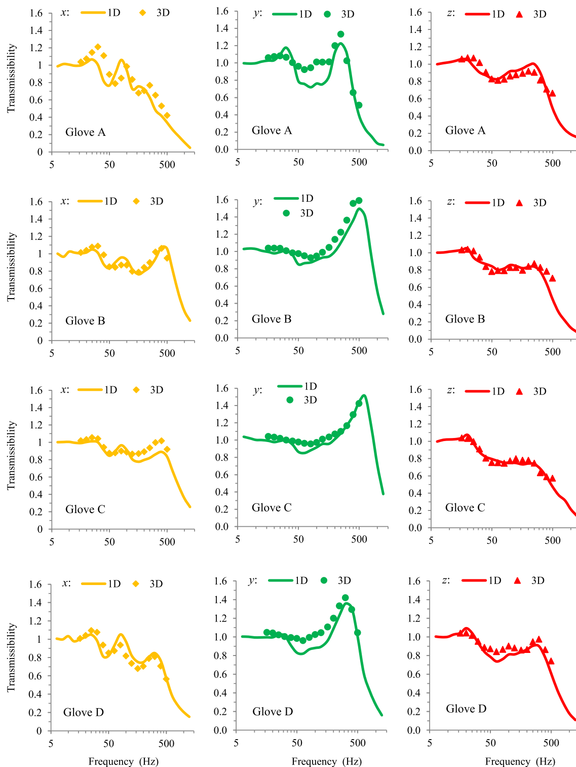
Fig. 9. Comparisons of the transmissibility spectra of the gloves measured on a 1-D test system with those measured on a 3-D vibration test system (McDowell et al., 2013a).
