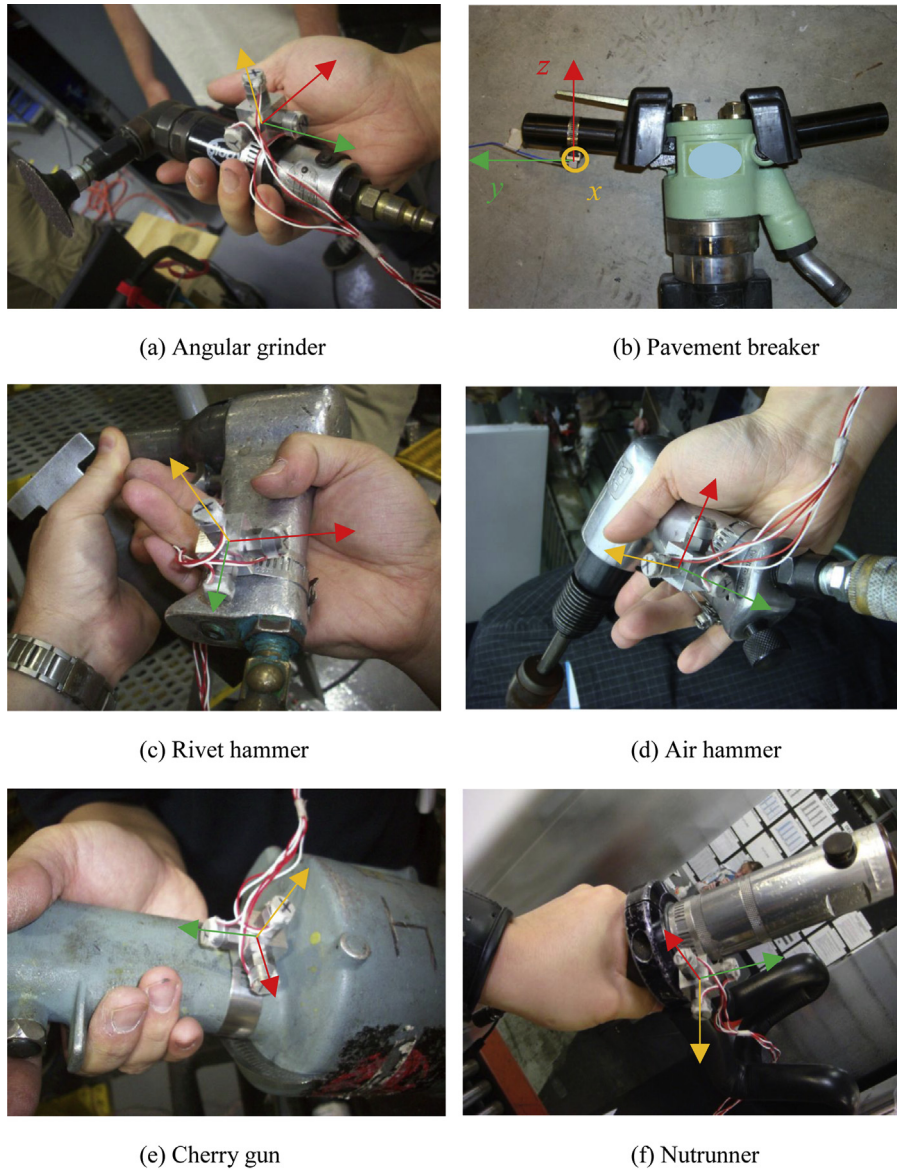
Fig. 7. Examples of accelerometers mounted on several tools and the hand grip postures in the measurements of tool vibrations.
