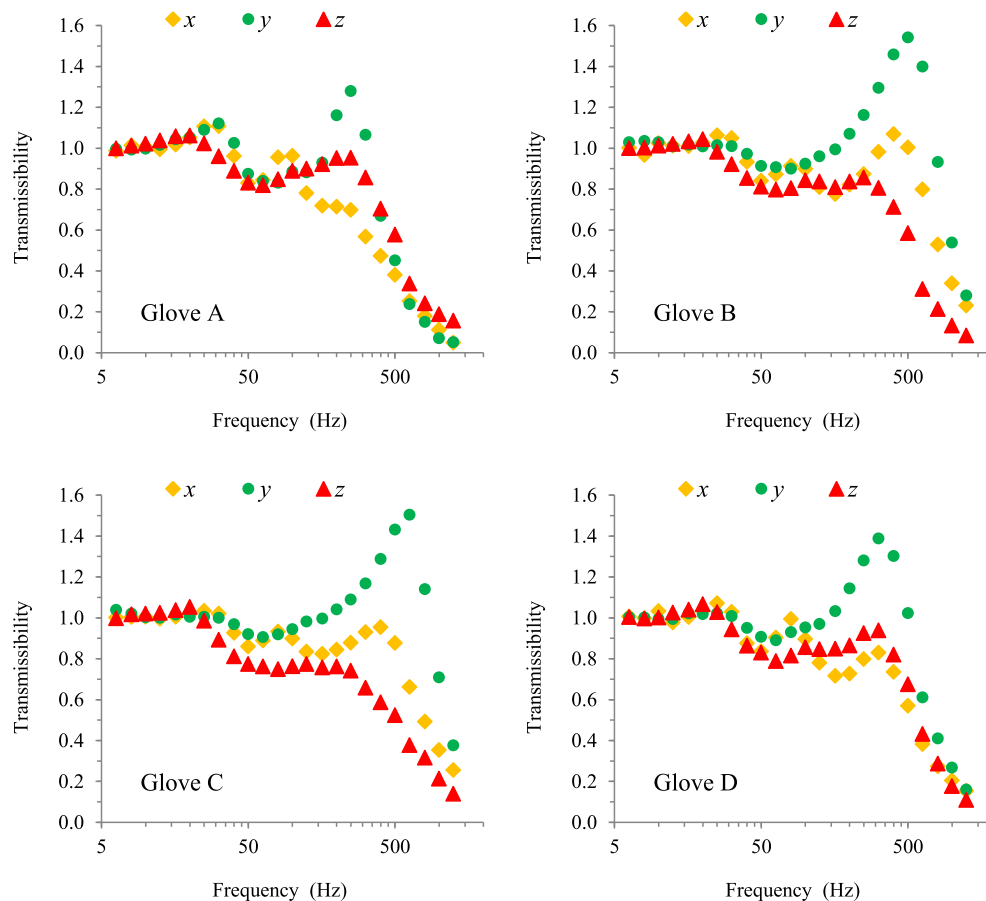
Fig. 10. Vibration transmissibility spectra of the four gloves synthesized using the data measured at the palm of the hand in the three orthogonal directions.
