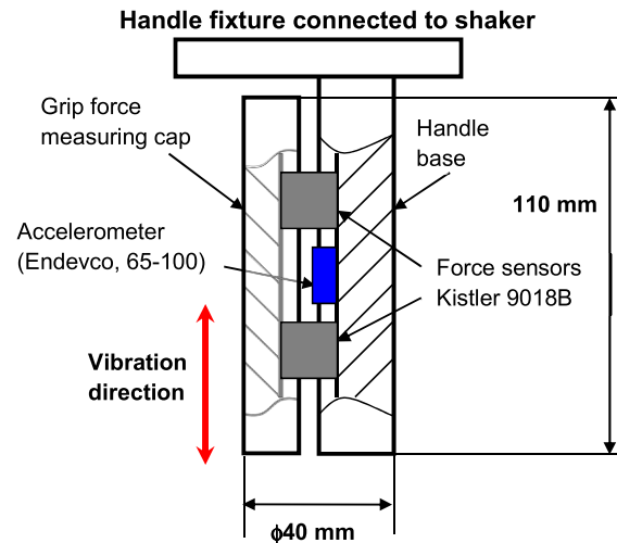
Fig. 5. A sketch of the instrumented handle for the measurement of glove transmissibility in the y direction.
