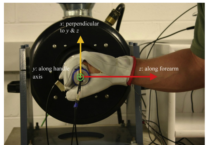
Fig. 6. The measurement of glove transmissibility at the palm in the y direction using a palm adapter on a 1-D vibration test system.
