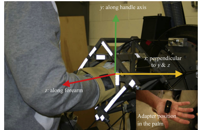
Fig. 2. The measurements of glove transmissibility spectra at the palm of the hand in the three orthogonal directions (3-D: x, y, and z) using a palm adapter on a 3-D hand-arm vibration test system (McDowell et al., 2013a).
