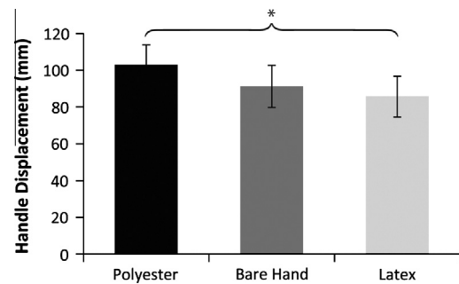
Fig. 6. Handle displacement decreased with increasing COF at the grip interface. The polyester glove with the lowest COF condition resulted in the greatest handle displacement until stabilization of the perturbed handle compared to latex glove condition ( p = 0.002 ). Error bars represent \pm one standard error. A star indicates a statistically significant difference.
