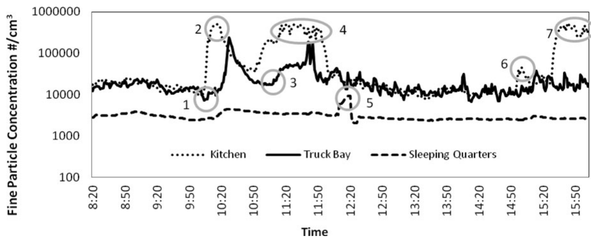
FIGURE 1. Number concentration of submicron particles measured with the P-Trak at three different areas at Firehouse B. Peak values are numbered in order of their chronological appearance.
