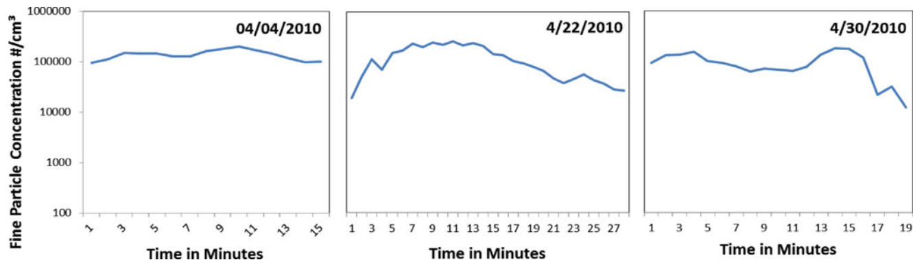
FIGURE 2. Number concentration of submicron particles measured with the P-Trak during three overhaul events at stated dates. (color figure available online)
