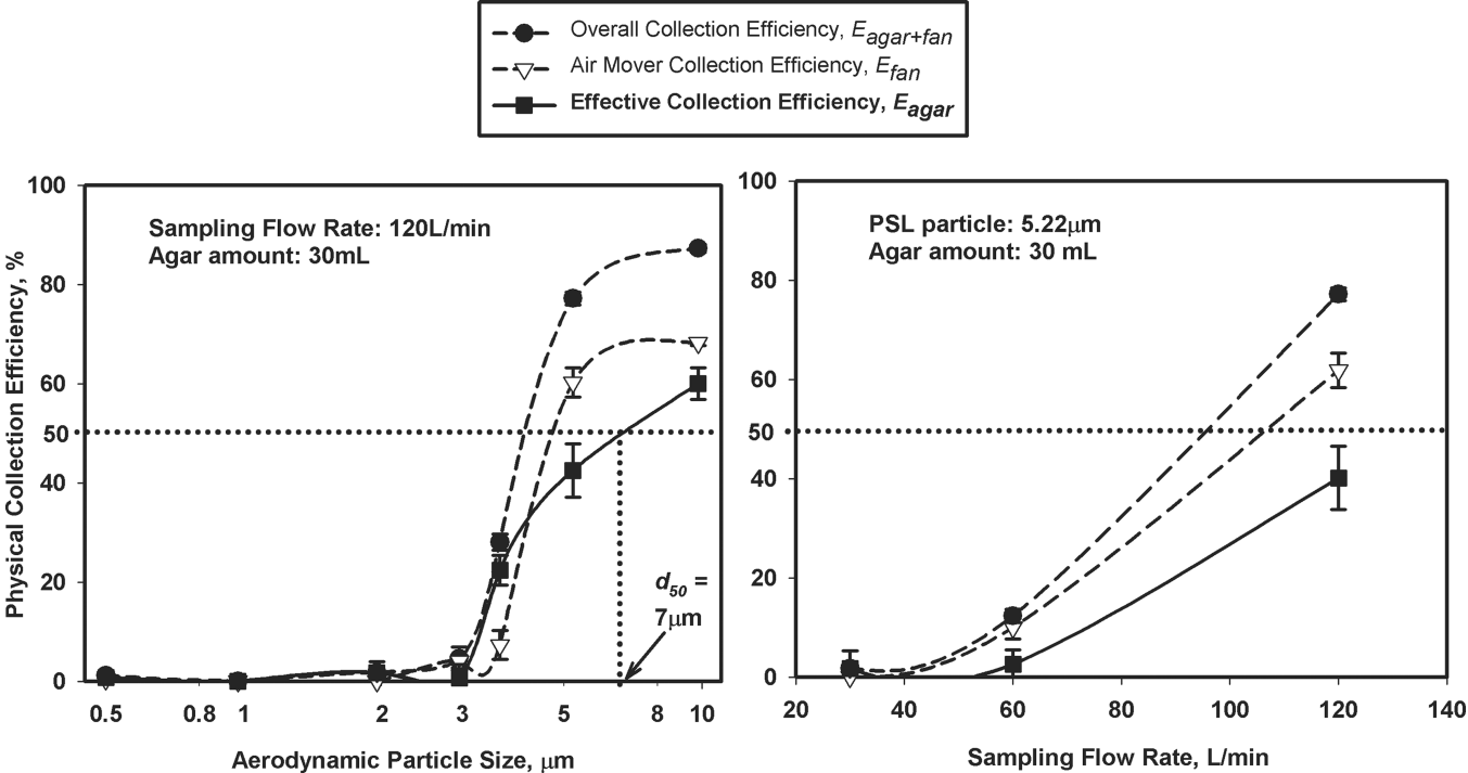
FIG. 3. Physical collection efficiencies of BioCulture microbial sampler at different sampling conditions. The data represent averages from three repeats and error bars stand for 1 standard deviation.
