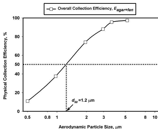
FIG. 8. Physical collection efficiency of RCS High Flow microbial sampler. Data represent averages from three repeats and error bars stand for 1 standard deviation.
