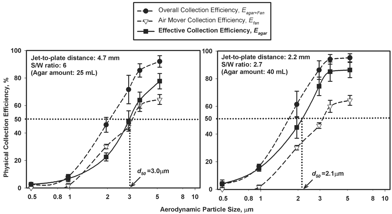
FIG. 6. Physical collection efficiencies of SAS Super 180 microbial sampler at different jet-to-plate distances. Data represent averages of three repeats and error bars stand for 1 standard deviation.
