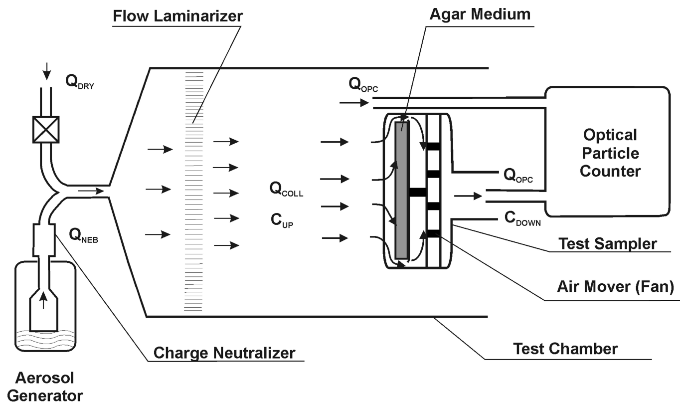
FIG. 1. A schematic representation of the experimental setup.
