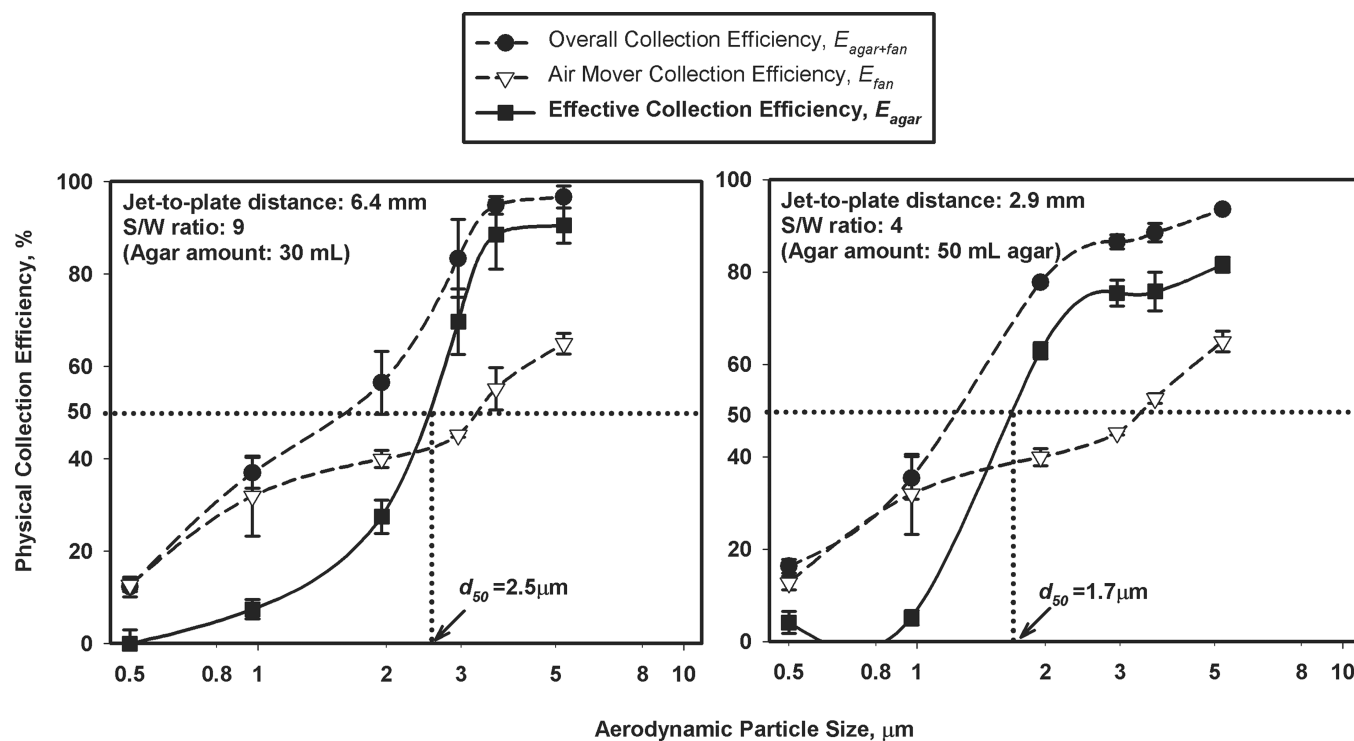
FIG. 4. Physical collection efficiencies of MAS-100 microbial sampler at different jet-to-plate distances. The data represent averages from three repeats and error bars stand for 1 standard deviation.
