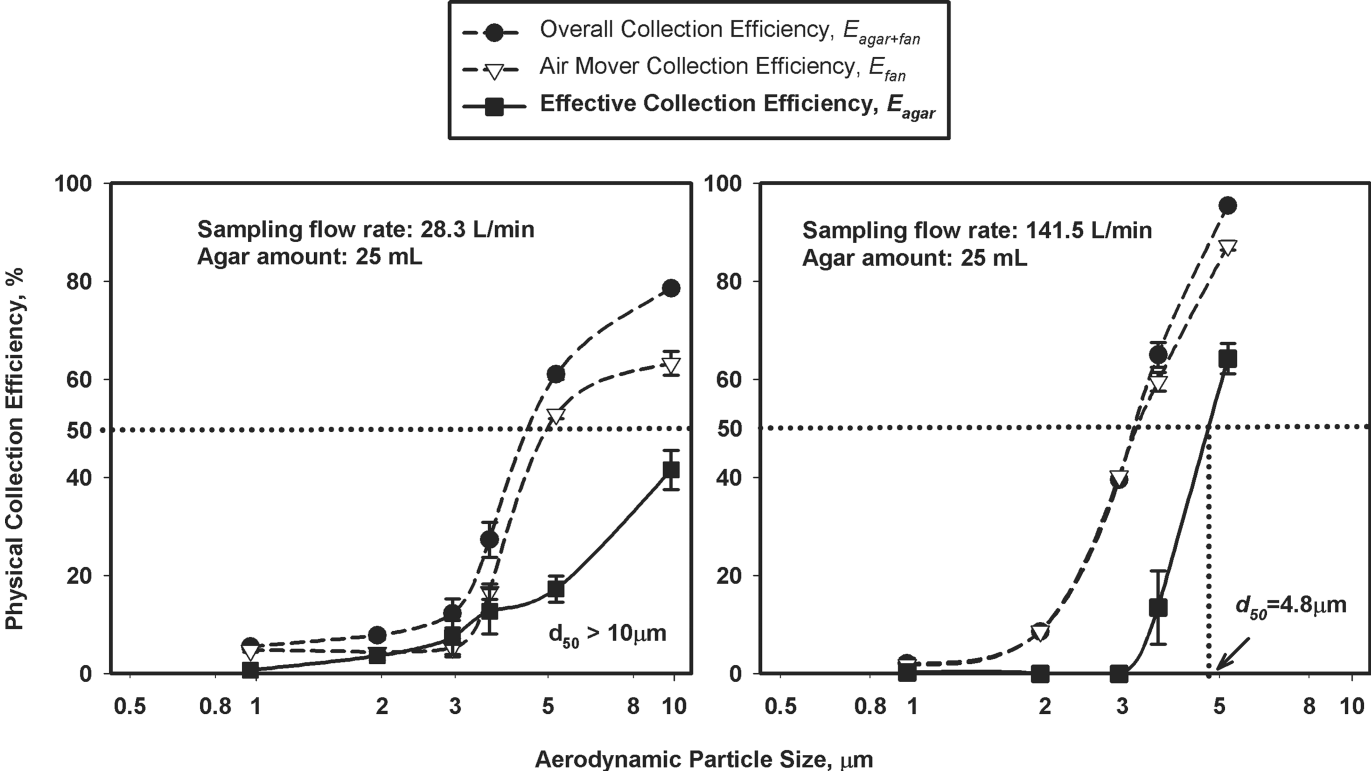
FIG. 2. Physical collection efficiencies of SMA MicroPortable microbial sampler at different sampling conditions. Data represent averages of three repeats and error bars stand for 1 standard deviation.
