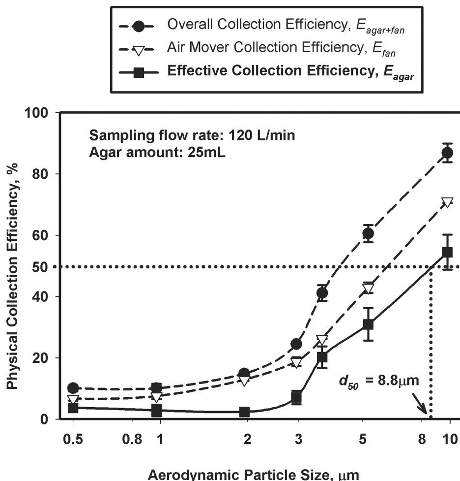
FIG. 5. Physical collection efficiencies of Microflow microbial sampler. Data represent averages of three repeats and error bars stand for 1 standard deviation.
