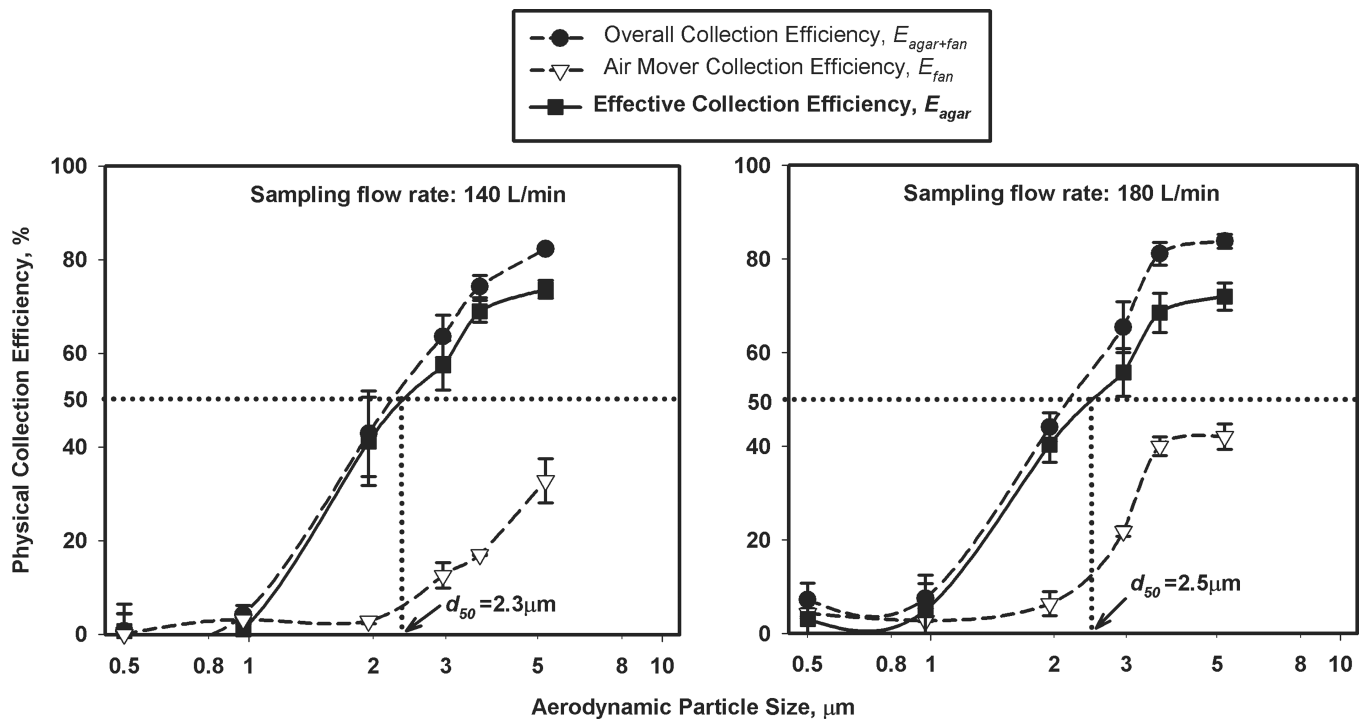
FIG. 7. Physical collection efficiencies of Millipore Air Tester at different sampling flow rates. Data represent averages of three repeats and error bars stand for 1 standard deviation.
