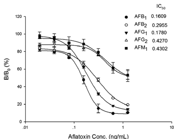
Figure 2. Cross-reactivity of VHH-based ELISA toward aflatoxin B 1 (●), B 2 (○), G 1 (▼), G 2 (△), and M 1 (■). Each result is represented as an average \pm standard deviation of three replicates.
