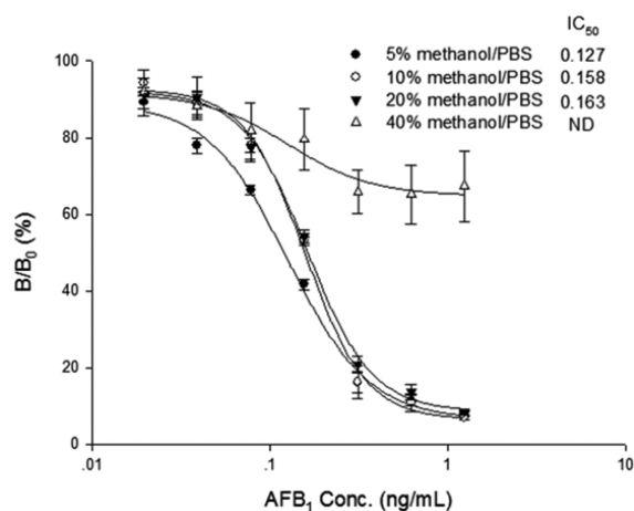
Figure 3. Performance of the VHH-based ELISA under 5% (●), 10% (○), 20% (▼), and 40% (△) methanol–PBS. Data are represented as an average \pm standard of three replicates.
