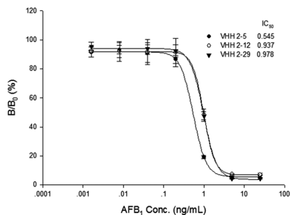
Figure 1. Inhibition curves of VHH-based ELISA with VHH 2-5 (●), VHH 2-12 (○), and VHH 2-29 (▼) antibodies as coating antigen. Each value is the average of three replicates \pm standard deviation. % B/B0 = [Absorbance (calibrator, control, or unknown)/Absorbance (blank)] \times 100.
