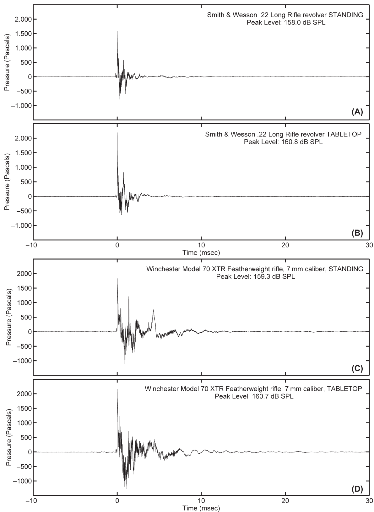
Figure 2. Impulse waveform comparisons for the Smith & Wesson .22 long rifle revolver (A, B) and the Winchester Model 70 XTR Featherweight rifle (C, D); shot from the standing (A, C) and the tabletop (B, D) shooting positions.
