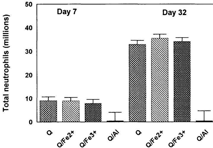
Fig. 1. Neutrophil numbers in lavage 7 and 32 days post-instillation of 1 mg metal-treated quartz (geometric mean and s.d.).
