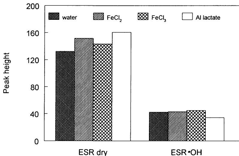
Fig. 2. Electron spin resonance (ESR) measurements as peak heights from 50 mg dry quartz samples and \cdot\text{OH} radical activity from 10 mg quartz samples in the presence of DMPO and \text{H}_2\text{O}_2 (mean of 3 experiments).
