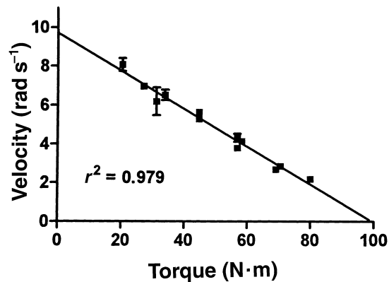
Figure 3 Torque-velocity relationship for 12 different loads selected at random for one subject. The data are presented as mean \pm standard deviation for three maximal efforts.
