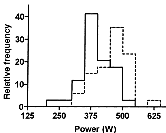
Figure 9 Relative frequency histogram for maximal power output of all subjects. Dashed line, before fatigue protocol; solid line, after fatigue protocol.
