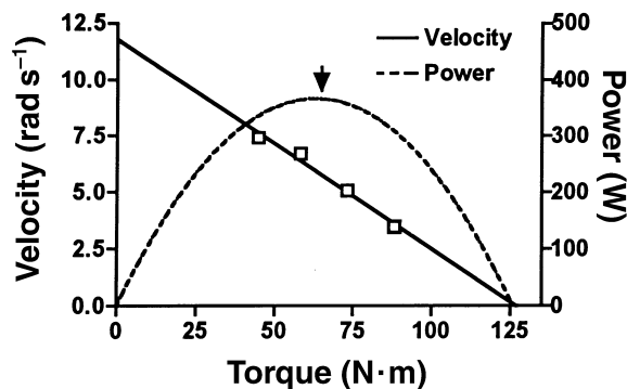
Figure 2 Torque-velocity and torque-power relationships. The squares represent the maximal velocities of knee movement at each of the four loads for one subject. The data are presented as mean \pm standard deviation for three maximal efforts. Power was calculated from the torque-velocity data. The arrow indicates calculated maximal power.
