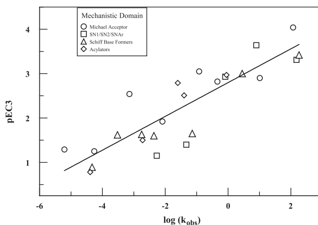
Fig. 3. \log(k_{\text{obs}}) versus pEC3 for the MA, Aca, SBF and \text{S}_{\text{N}}1/\text{S}_{\text{N}}2 domains listed in Table 1. There was strong correlation ( R^2 = 0.76 ) between PDA reactivity and potency in the LLNA. The seven chemicals which did not react with PDA and three chemicals without LLNA data were not included in this plot. \text{pEC3} = \log\{\text{MW}/\text{EC3}\} .
