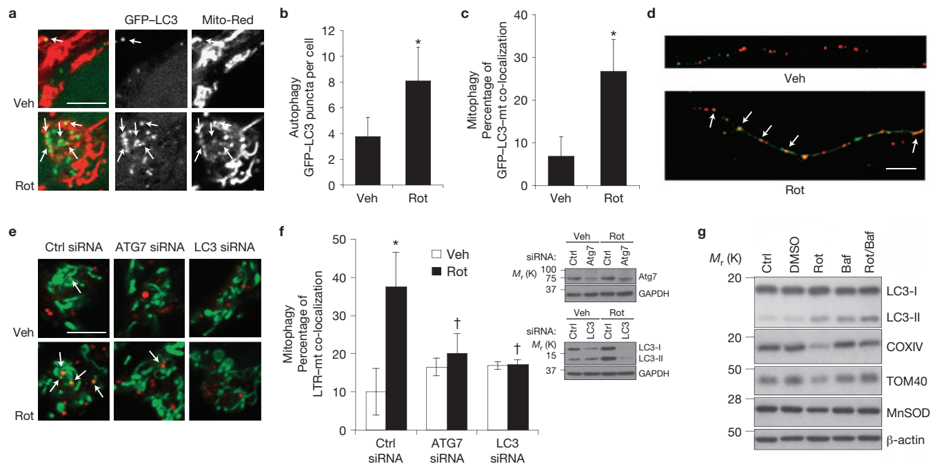
Figure 1 Rotenone-induced mitophagy. ( a–d ) Rotenone (Rot) increased the number of GFP-LC3 puncta and the level of co-localization with mitochondria (arrows) in SH-SY5Y cells ( a–c ; 1 \mu M) and primary cortical neurons ( d ; 250 nM), quantified in Fig. 3f and Supplementary Fig. S1b,c. Veh, vehicle. ( e,f ) Rotenone increased delivery of MitoTracker Green-stained mitochondria (mt) to LysoTracker Red (LTR)-stained lysosomes, inhibited by siRNA knockdown of ATG7 or LC3 in SH-SY5Y cells. Ctrl, control. Right: RNAi knockdown. ( g ) Rotenone decreased
