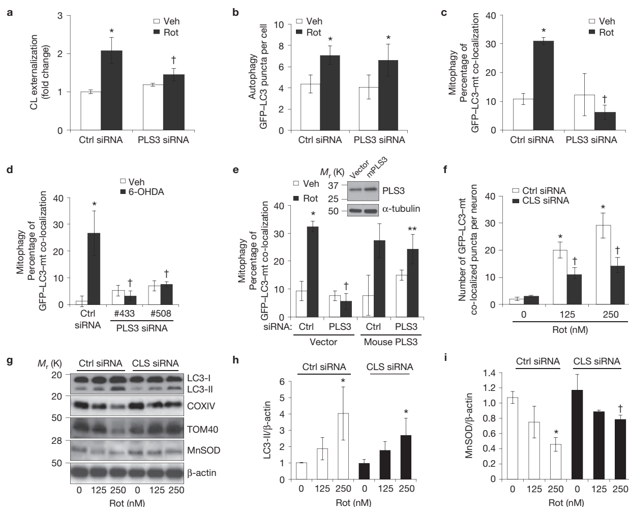
Figure 3 RNAi knockdown of CL enzymes attenuates CL exposure and mitophagy. ( a–e ) SH-SY5Y cells expressing control (Ctrl) or scramblase-3 siRNA #508 (PLS3 siRNA) for 72 h were stained with MitoTracker Green FM, a transmembrane potential-independent dye, and treated with rotenone (Rot; 1 \mu M). Veh, vehicle. ( a ) Anionic phospholipids exposed to the outer surface of isolated mitochondria were quantified by flow cytometry for Alexa 647–annexin V binding. ( b–d ) PLS3 knockdown had no effect on rotenone-induced autophagy ( b ), but decreased mitophagy in SH-SY5Y cells treated with rotenone ( c ; 1 \mu M) or 6-OHDA ( d ; 120 \mu M). ( d,e ) The effects of PLS3 siRNA were recapitulated using a second siRNA #433 ( d , Supplementary Fig. S3b,g), and reversed by transfection with
