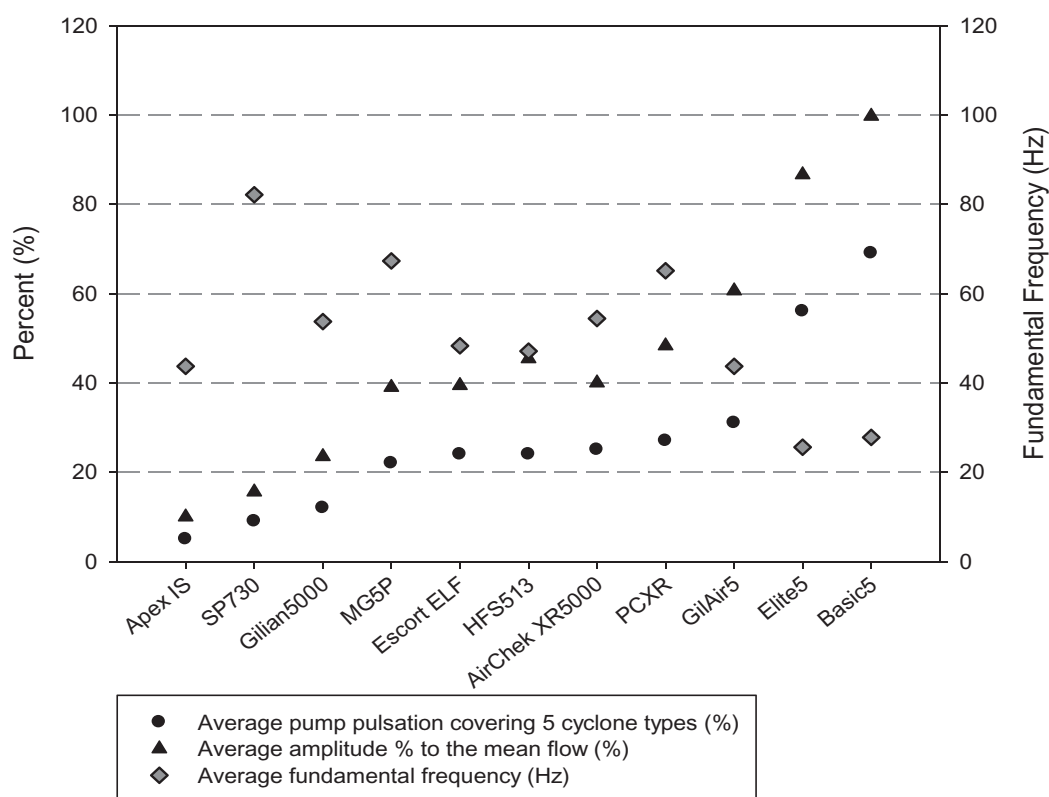
5 Average PP (%), fundamental frequency of pulses (Hz), and average amplitude of pulses compared to the associated mean flows (%) for the medium volumetric flow rate pumps.
