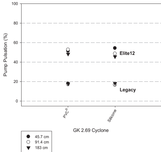
7 PPs with various tubing materials and lengths (PVC a : pulsation measurements by NIOSH; PVC b : pulsation measurements by IFA). Note that the two square solid dots for the Basic5 and Apex IS are pulsations with a flow resistor.
