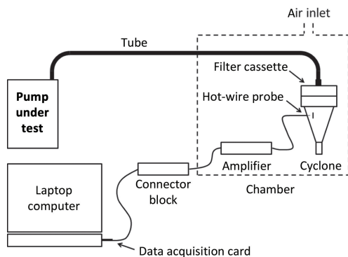
2 Experimental set-up (NIOSH).
