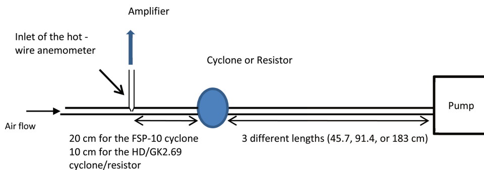
3 Experimental set-up for pulsation measurements (IFA).
