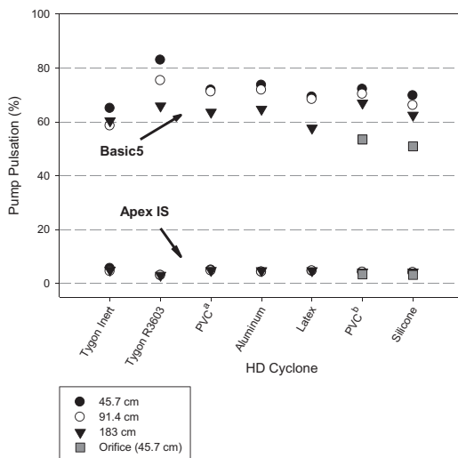
7 PPs with various tubing materials and lengths (PVC a : pulsation measurements by NIOSH; PVC b : pulsation measurements by IFA). Note that the two square solid dots for the Basic5 and Apex IS are pulsations with a flow resistor.
