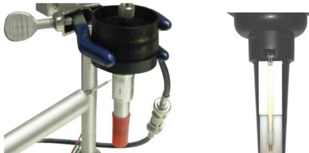
1 Hot-wire anemometer probes: placed near the inlet of a cyclone (left); held in a custom bracket and cemented onto a cyclone (right).
