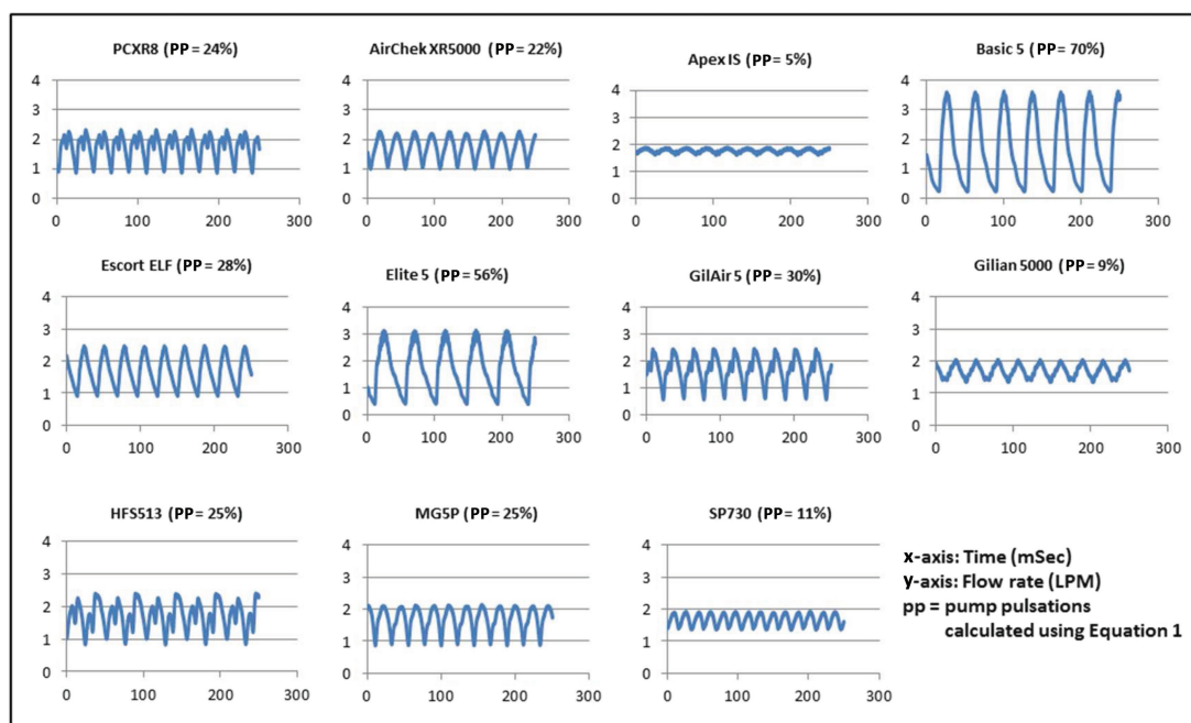
4 Example of PPs (medium volumetric flow rate pumps connected to the DO cyclone).
