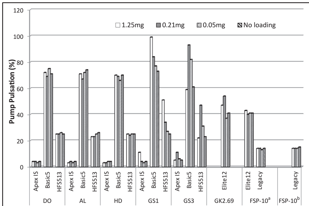
6 Comparison of PPs with different filter loading (Note that the nominal flow rate for the FSP-10 a and FSP-10 b was 10 and 11.2 l min -1 , respectively.).
