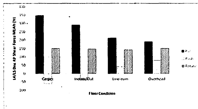
Figure 10: L4/L5 Anterior posterior (AP) shear force by task and floor condition
