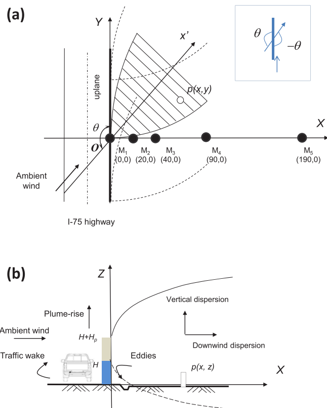
Fig. 1. a) Cartesian coordinates of the highway and monitoring stations (in m) showing geometric relationships between air plumes (solid and dashed lines), wind, traffic and M_1 – M_5 transect; b) black carbon transport in cross-section with major mechanisms marked for a receptor p(x,z) in a flat open area.
