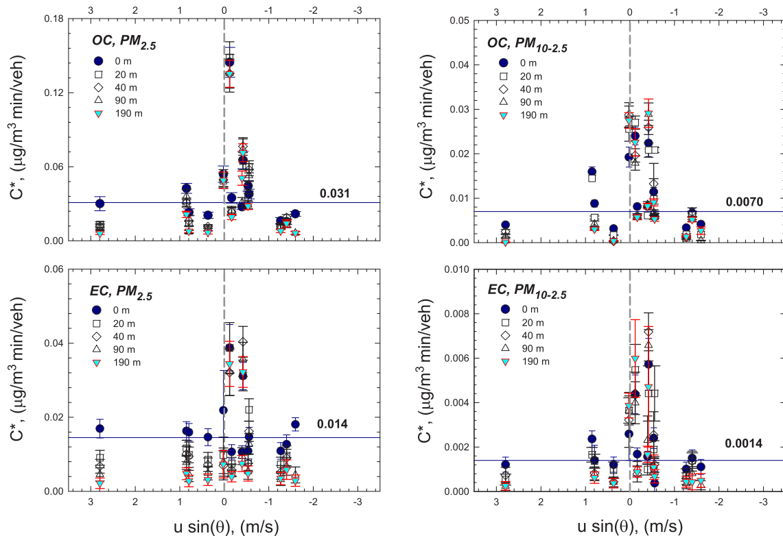
Fig. 6. C_{OC}^* and C_{EC}^* as a function of u \sin \theta . Horizontal bar and number indicate C_{OC}^* or C_{EC}^* averages of samples at M_1 ( x = 0 ) excluding those under oblique low upwinds. Error bar is 1\sigma uncertainty C_{OC}^* and C_{EC}^* and are normalized concentrations to the traffic flow.
