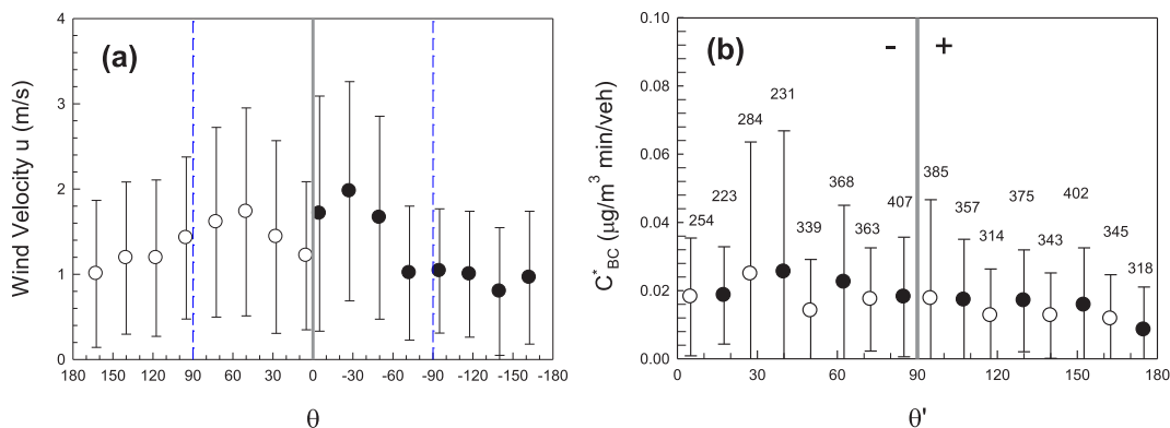
Fig. 3. Statistics of u and C_{BC}^* at M_1 station for the monitoring periods. Numbers of minutely measurements are marked. “+” and “-” indicate wind along and counter traffic in uplane. \theta is the angle between road and wind direction. \theta' is the conversion of \theta to describe the traffic wake effect. C_{BC}^* is BC concentration normalized to the traffic flow.
