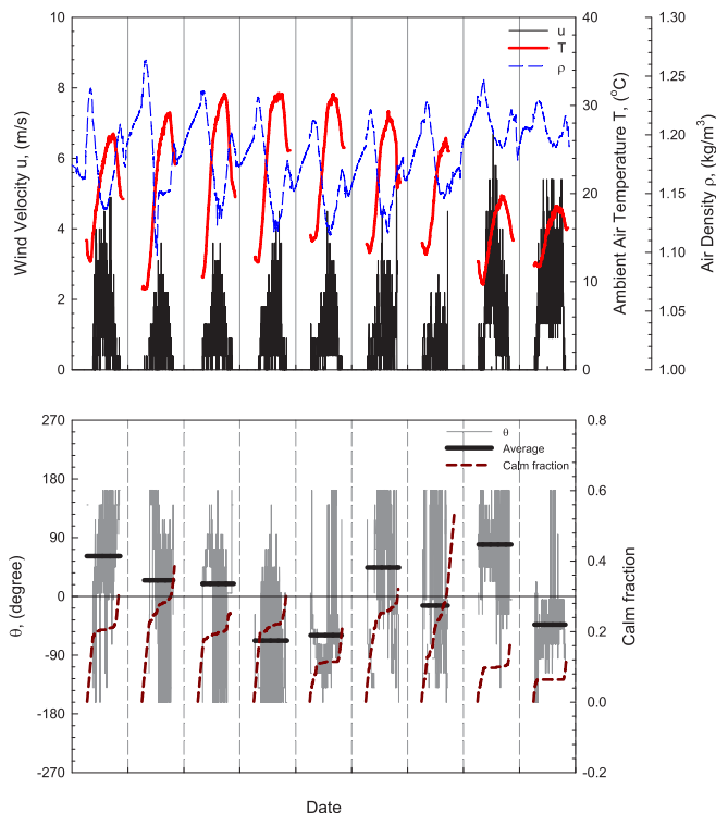
Fig. 2. Diurnal variations of u , \theta , T , \rho , and daily accumulative calm fraction. \theta is the angle between the road and wind direction in Fig. 1.
