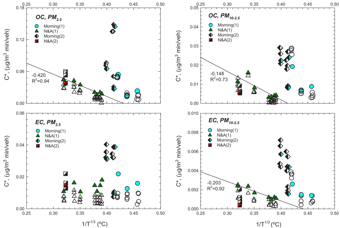
Fig. 7. C_{OC}^* and C_{EC}^* variations with temperature at M_1 (solid symbols) and M_2 – M_5 (open). Labels in legend: N&A – noon–afternoon; (1) – Gaussian dispersion; (2) – non-Gaussian dispersion. Regression slope and R^2 are marked.
