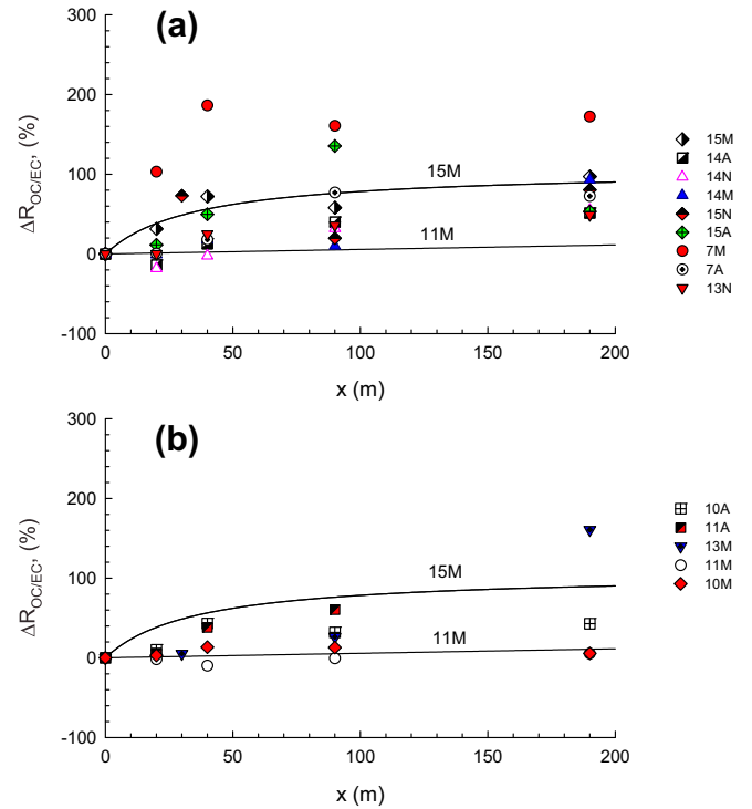
Fig. 10. % change of OC and EC in PM 2.5 in roadside transport for the two groups: A) Gaussian dispersion; b) uniform distribution. 15M and 11M lines are based on Eq. (6).
