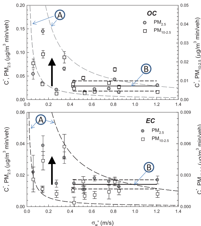
Fig. 12. Variations with \sigma_w' , the overall wind velocity variance, for OC and EC in \text{PM}_{2.5} and \text{PM}_{10-2.5} . Model lines: A) C^* \sim 1/\sigma_w' of Venkatram et al. (2007); B) C^* \sim p(\theta) line ( m \pm 1\sigma ). Arrows indicate possible meandering effect.
