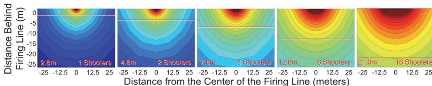
Figure 2. The 85-dBA foul line for a .270 caliber A-Bolt Medallion Rifle with muzzle brake moves from less than 3 meters to 21 meters as the number of shooters increases from 1 to 16. The spacing between shooters is 1 meter and the number of shots fired is 25.
