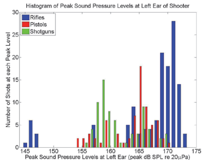
Figure 1. The peak sound pressure levels ranged between 145 and 173 dB for a microphone close to the left ear of the shooter.
