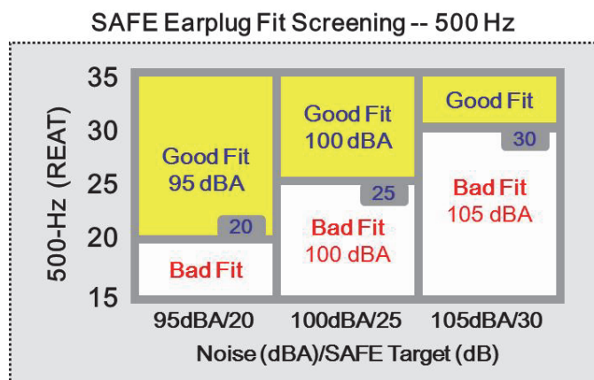
Figure 2. SAFE-500 conversion diagram for use in hearing protection program surveillance
