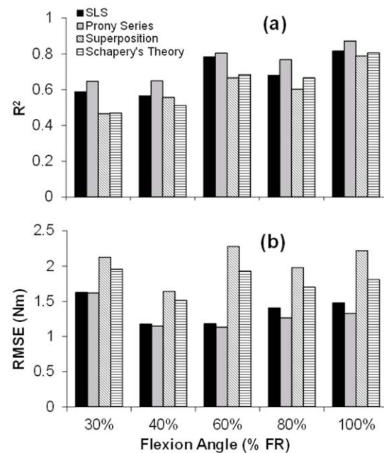
Figure 5. Mean measures of viscoelastic model prediction quality: (a) R^2 and (b): root-mean-square errors (RMSE).
