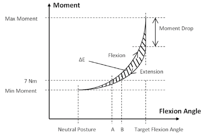
Figure 2. Illustration of a hysteresis loop. The highlighted area ( \Delta E ) denotes the dissipated energy; NZ in flexion (extension) is the distance between point A (point B) and the neutral posture. Target lumbar flexion angle = 30, 40, 60, 80, or 100% FR. doi:10.1371/journal.pone.0048625.g002
