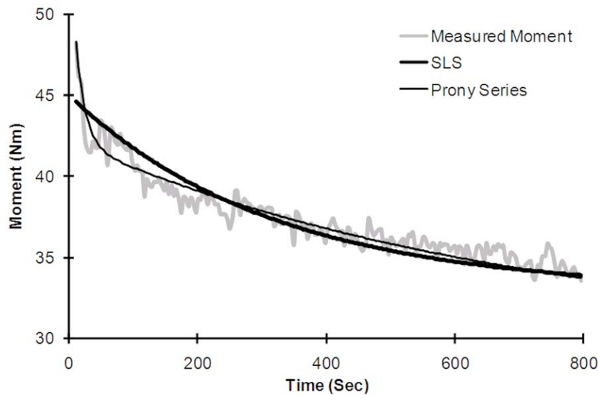
Figure 7. Fast and slow phases of moment drop during the load-relaxation period. Representative data are shown, and which indicate the advantage of the Prony Series over the SLS model for predicting measured behaviors. Results are for a 100% FR exposure. doi:10.1371/journal.pone.0048625.g007
