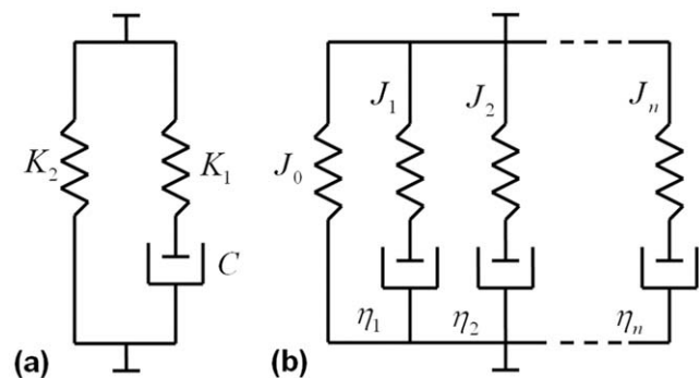
Figure 3. Illustration of two Kelvin-solid models: (a) SLS model (b) Prony Series model. Each spring and damper in series represents a Maxwell model. For clarity, linear rather than rotational components are illustrated. doi:10.1371/journal.pone.0048625.g003
