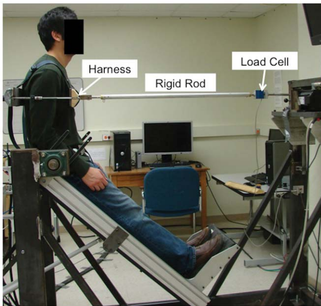
Figure 1. Experimental setup for load-relaxation test (60% FR angle condition illustrated). doi:10.1371/journal.pone.0048625.g001
