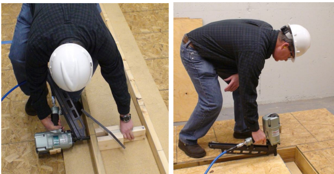
Figure 3. Wall-building task, with user holding the sham stud/shielding fixture with the opposite hand (left). The nails protruded through the gap between the slotted side brackets of the device into which the shield was inserted. The sham stud held in the
