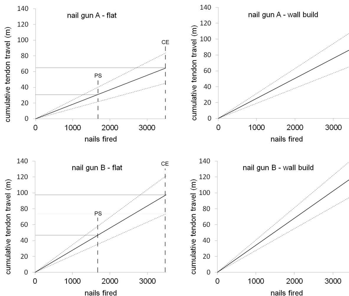
Figure 6. Predicted cumulative tendon travel exposure as a function of the number of nails fired, for combinations of nail gun and task (flat = flat nailing, wall build = wall building). The thin dotted lines outline the 95% confidence interval band for these predictions. Vertical dashed lines (flat nailing graphs) represent high production work estimates of nails/worker/day based on productivity standards ( PS ) and contractor estimate ( CE ), as described in the Discussion .
