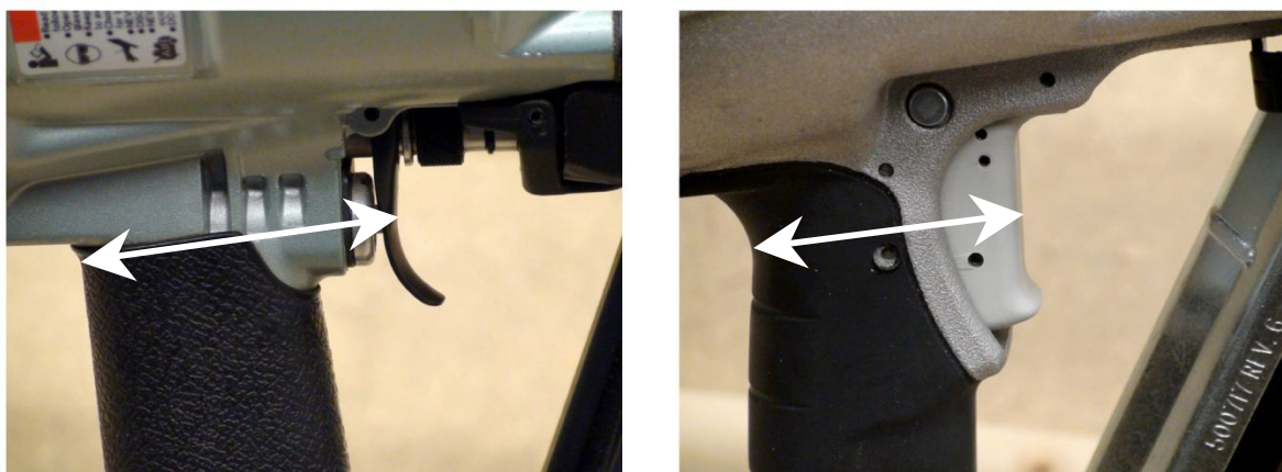
Figure 1. Triggers for nail gun A (left) and nail gun B (right). The trigger reach distance (shown with arrows) for trigger A was 66 mm; and for trigger B was 55 mm.
