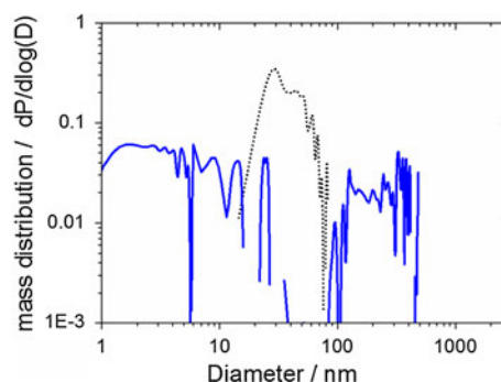
Fig. 2 Positive and negative controls for the size distribution of suspended sanding fragments. Water as negative control ( blue solid line ); a CNT suspension as positive control was measured after the same de-agglomeration protocol ( black dotted line ). (Color figure online)
