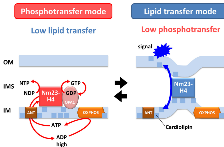
FIGURE 8. Model of Nm23-H4 as a bifunctional nanoswitch. In phosphotransfer mode (elements in red/brown/orange ), Nm23-H4 only binds to mitochondrial IM and thus maintains phosphotransfer activity, although lipid transfer activity is low or absent. In this mode, Nm23-H4 regenerates NTP (mainly GTP) in the IMS, in particular for local use, e.g. by the interacting GTPase OPA1. Nm23-H4 also channels ADP via ANT into the matrix space for stimulation of respiration and ATP regeneration (8). In the lipid transfer mode (elements in light and dark blue ), the symmetrical Nm23-H4 hexamers have to be fully membrane-bound, i.e. attached simultaneously to IM and OM, virtually cross-linking these two membranes (6, 8). This will inhibit phosphotransfer activity but allow for intermembrane lipid transfer, in particular of cardiolipin, whose exposure at the mitochondrial surface is suggested to have signaling character. The switch between the two modes may depend on the availability/accessibility of cardiolipin and other anionic phospholipids in the IM outer leaflet and the OM inner leaflet (for further details see text). OXPHOS , oxidative phosphorylation.
