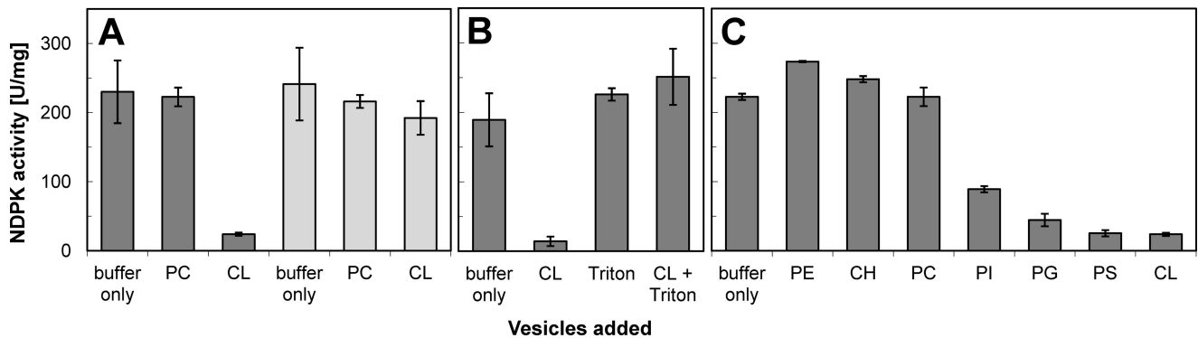
FIGURE 3. Nm23-H4 phosphotransfer activity is inhibited by anionic phospholipids. A, phosphotransfer activity of Nm23-H4 WT (dark gray bars) is inhibited to about 90% by binding of anionic CL (100 \mu g/ml), whereas zwitterionic PC (100 \mu g/ml) has no effect. By contrast, phosphotransfer activity of membrane binding-deficient Nm23-H4 R90D mutant (R90D, light gray bars) is not affected by CL. B, inhibition of Nm23-H4 WT phosphotransfer activity by CL can be relieved by addition of detergent (0.5% Triton X-100). C, phospholipids with neutral net charge, PC, and phosphatidylethanolamine (PE), or cholesterol (CH) do not inhibit Nm23-H4 phosphotransfer, although anionic phospholipids phosphatidylinositol (PI), phosphatidylglycerol (PG), phosphatidylserine (PS), and CL are inhibitory (all lipids at 100 \mu g/ml). Note: under conditions used in this assay, Nm23-H4 is quantitatively bound at both binding faces to lipid vesicles (8). Furthermore, this inhibition profile parallels the binding of Nm23-H4 to these lipids (see Fig. 2 in Ref. 8). Data are means \pm S.D., n = 3 .
