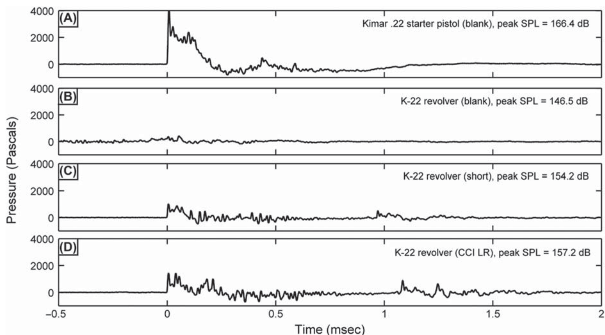
Figure 2. Composite waveforms recorded from the shooter's left ear. Panel (A) Kimar .22 starter pistol firing Winchester blanks; (B) K-22 Masterpiece firing Winchester short blanks; (C) K-22 Masterpiece revolver firing Winchester shorts; and (D) K-22 Masterpiece revolver firing CCI Long Rifle ammunition. Sound pressure levels and L_{eqA8} are discussed in the text and summarized in Tables 1 and 2.
