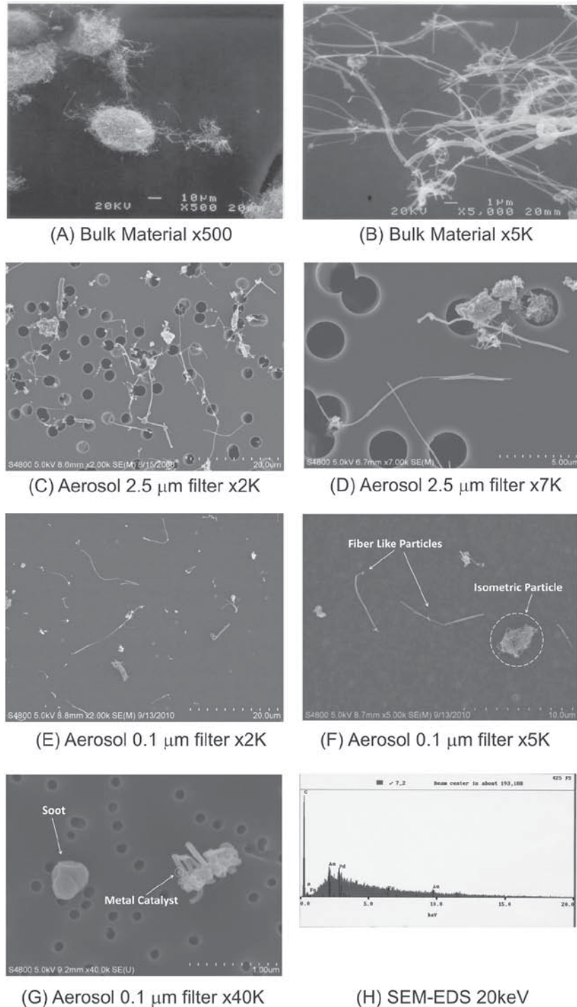
Figure 1. Scanning Electron photomicrographs of MWCNT's: (A) bird-nest configuration in bulk material (non-dispersed), bar length = 10 µm; (B) bundled-together formation in bulk material (non-dispersed), bar length = 1 µm; (C-G) representative samples of aerosol particles generated from the acoustic disperser, collected using two different pore size filters (2.5 vs. 0.1 µm) with various magnifications (×2k-×40k), the full range of the tick marks are 20, 10, 5, and 1 µm, respectively; (H) SEM-EDX analysis indicates that the particles contain primarily carbon (gold and palladium are elements in the coating material).
