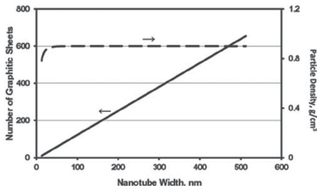
Figure 11. The relationship of number of sheets and fiber density (with voids) of a multi-walled nanotube with respect to its tube width. The values of number of sheets and particle density were calculated based on the measurements of the nanotube from a high-resolution TEM images (Porter et al., 2010; Figure 1), in which the width of the inner hollow core ( W_c ) = 5.385 nm, the thickness of a graphitic sheet ( W_T ) = 0.166 nm, and the distance between two graphitic sheets ( W_D ) = 0.222 nm. The material density of graphite was provided by the manufacturer as 2.1 \text{ g/cm}^3 .
