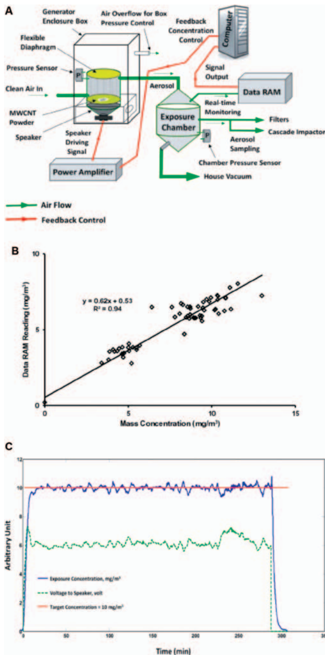
Figure 2. (A) Schematic of a NIOSH MWCNT exposure system including an acoustical generator, exposure (sampling) chamber, and a feedback system; (B) Relationship between the readings from Data RAM and mass concentrations gravimetrically measured from PTFE filters; and (C) A real-time profile of speaker driving voltage and MWCNT concentration in the chamber with a target concentration of 10 mg/m 3 . The actual concentration (mean \pm standard deviation) was 10.02 \pm 0.19 mg/m 3 with a daily range of 9.4–10.5 mg/m 3 . Also shown is the output voltage to the speaker of the acoustic generator. The inverse relationship between the voltage profile and the concentration profile indicates that the feedback system worked as expected.
