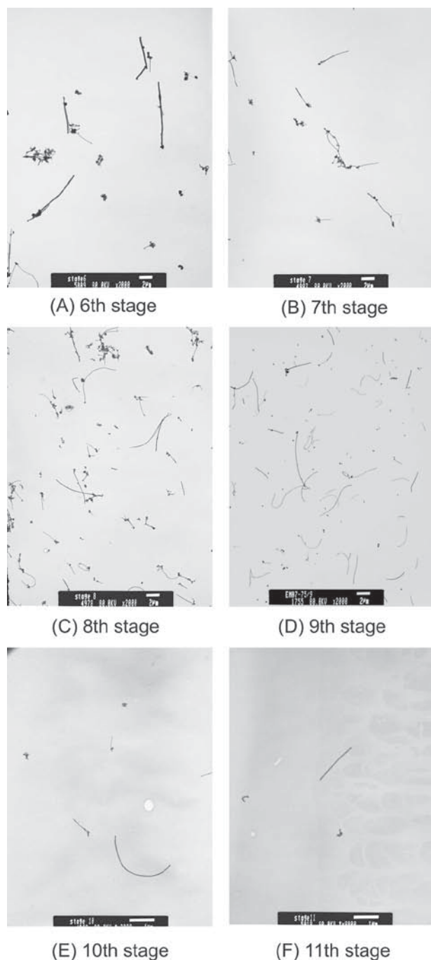
Figure 7. TEM photomicrographs of particles collected on the grids of MOUDI stages 6–11 (A–F). The scale bars are 2 \mu\text{m} on A–D and 1 \mu\text{m} on E–F. The 50% cutoff diameters, d_{50} , on stages 6–11 are 1.0, 0.56, 0.32, 0.18, 0.10, 0.056 \mu\text{m} , respectively.
