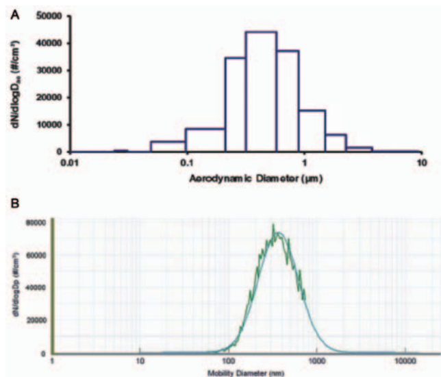
Figure 8. Representative number-based particle size distributions of the MWCNT aerosol obtained from two near-real-time instruments. (A) A histogram obtained from ELPI, with a count median of 0.45 \mu\text{m} (GSD = 2.09) and a number concentration of 3.4 \times 10^4 particles/ \text{cm}^3 , where N = number concentration and D_{ae} = aerodynamic diameter. (B) A zigzag curve obtained from SMPS, where D_p is the electrical mobility equivalent diameter. The smooth curve in (B) was compiled by assuming that the particle size follows a unimodal lognormal distribution. The count median is 360 \text{ nm} with a geometric standard deviation of 1.70. The number concentration is 4.2 \times 10^4 particles/ \text{cm}^3 .
