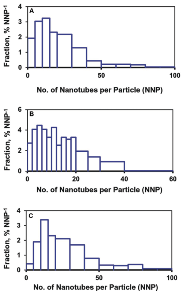
Figure 3. Graphical representation of the distribution of number of nanotubes per particle (NNP) in a MWCNT sample: (A) total particles, (B) fibrous particles and (C) isometric particles. The fraction per unit x-axis interval (% NNP -1 ) is plotted as the height of the histogram. Distribution of total particles (A) follows lognormal statistics with a count median NNP of 16 and a geometric standard deviation of 2.1.
