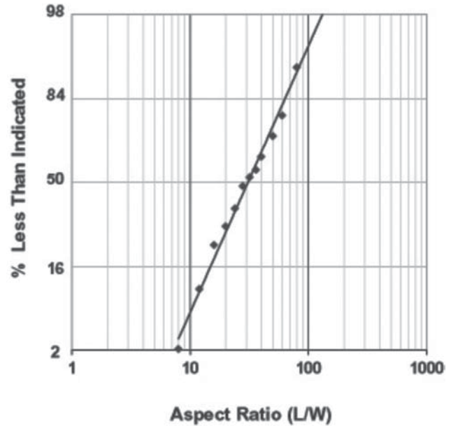
Figure 9. Cumulative distribution of the aspect ratio of the fiber-like particles shown with a log probability plot. The count median aspect ratio and geometric standard deviation are determined as 31.0 and 2.09, respectively.
