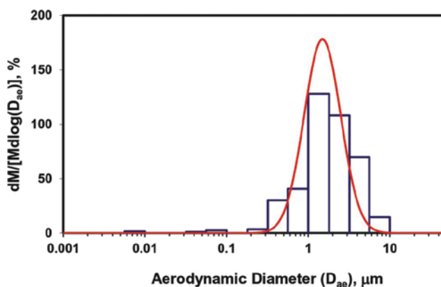
Figure 6. A typical particle size distribution of the MWCNT aerosol in the sampling chamber. The histogram shows the percent mass concentration per unit size interval ( M = mass concentration, D_{ae} = aerodynamic diameter) obtained from MOUDI and the curve indicates the expression of the primary size mode under the assumption of a lognormal distribution, which results in a MMAD of 1.50 \mu\text{m} and a GSD of 1.67. A mass mode of 1.34 \mu\text{m} and a count mode of 0.42 \mu\text{m} were qualitatively determined from the distribution.
