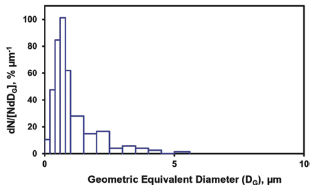
Figure 5. Number-based size distribution of the isometric particles in the MWCNT aerosol collected from the animal exposure chamber. The histogram shows the percent number concentration per unit size interval ( N = number concentration, D_G = geometric equivalent diameter). The distribution can be lognormally expressed with a count median diameter (CMD G ) of 0.90 \mu\text{m} and a geometric standard deviation (GSD) of 2.08.
