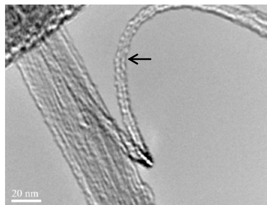
Figure 1: High-resolution transmission electron micrograph of SWCNTs. A representative crystalline structure of a bundle of SWCNT from HRTEM. Arrow shows the distinctive single-walled nanotube structure (two tubes bound together with each diameter about 2 nm).
