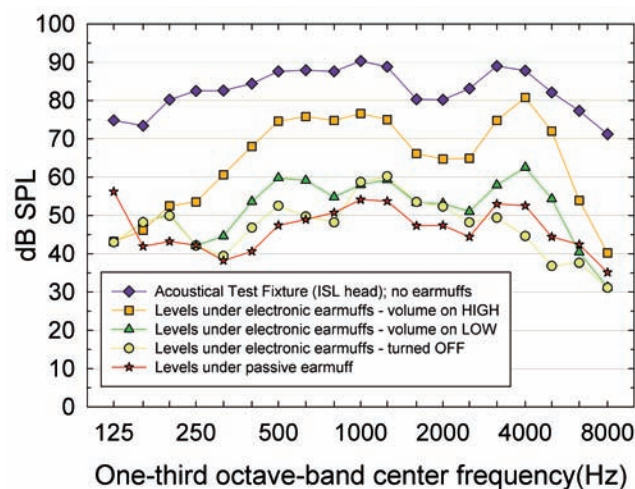
Figure 3. Measurements of HINT speech-shaped noise in the diffuse-field test chamber with the acoustical test fixture.
