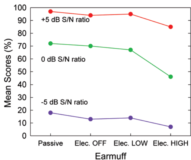
Figure 1. Graphic presentation of mean speech intelligibility scores for each earmuff condition with speech-to-noise ratio as the parameter.
