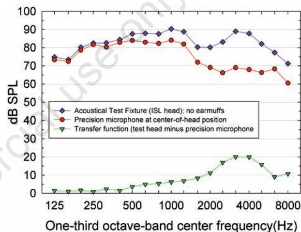
Figure 2. Measurements of HINT speech-shaped noise in the diffuse-field test chamber [overall level=90 dB(A)].
