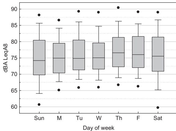
Figure 5. Daily sound levels ( \text{dBA Leq}_{A,8,\text{equiv}} ) by day of week. Figure details are similar to figure 4.
