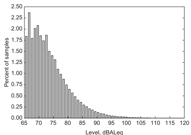
Figure 1. Histogram of \text{dBL}eq_{A,3.75} values above dosimeter threshold.
