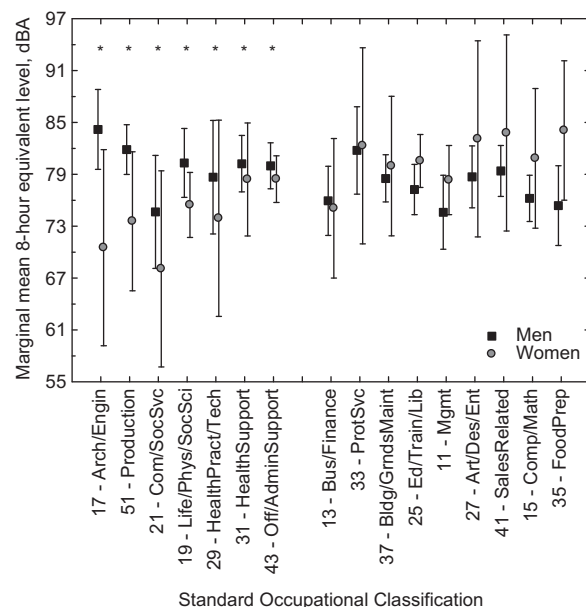
Figure 6. Marginal mean sound levels ( \text{dBA Leq}_{A,8,\text{equiv}} ) by BLS Standard Occupational Classification and gender, controlling for main effects of gender and self-reported history of work in noise. Error bars represent 95% confidence intervals for means, symbols (*) indicate significant interaction effects ( p < .05 ) by gender, after controlling for main effects.
