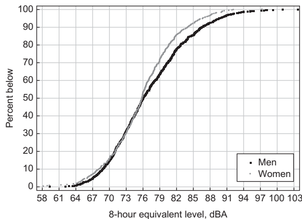
Figure 2. Cumulative distribution of overall daily sound levels ( \text{dBLeq}_{A,8,\text{equiv}} ) estimated from dosimeter runs.
