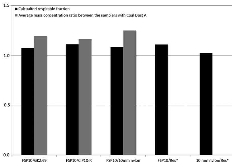
Fig. 8. Comparison calculated respirable fraction and average mass concentration ratio between the samplers with Coal Dust A.
