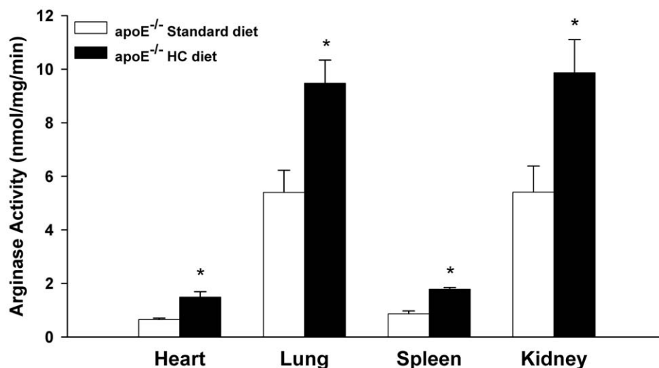
Figure 6. Induction of tissue arginase activities in \text{apoE}^{-/-} mice on HC diet. Values are means \pm SE for n=6 in each group. * p<0.05 vs standard diet. doi:10.1371/journal.pone.0015253.g006
