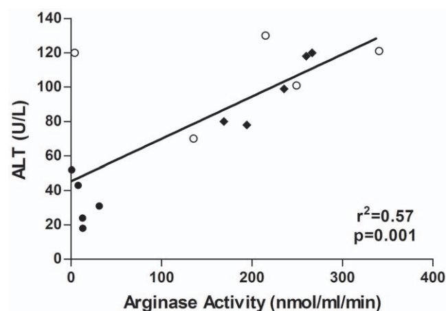
Figure 4. Correlation between activities of ALT and arginase in plasma of \text{apoE}^{-/-} mice on different diets. Regression analysis of ALT and arginase activities for the different diets ( n=5 in each group) is indicated by the solid line. Key to symbols: solid circles, standard diet; solid diamonds, HF diet; open circles, HC diet.
