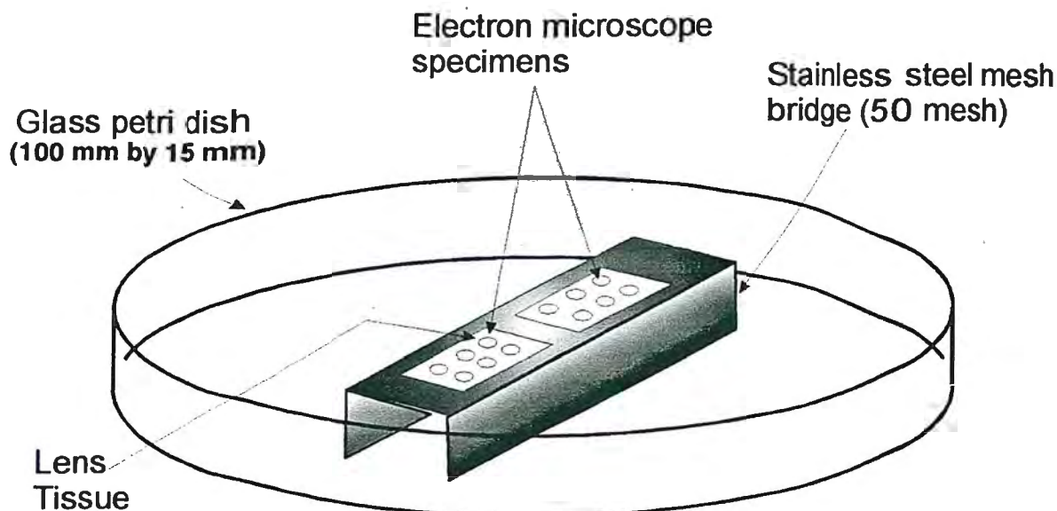
FIG. X1.2 Example of Design of Solvent Washer (Jaffe Washer). (Solvent is added until the meniscus contacts the underside of the stainless steel mesh.)
