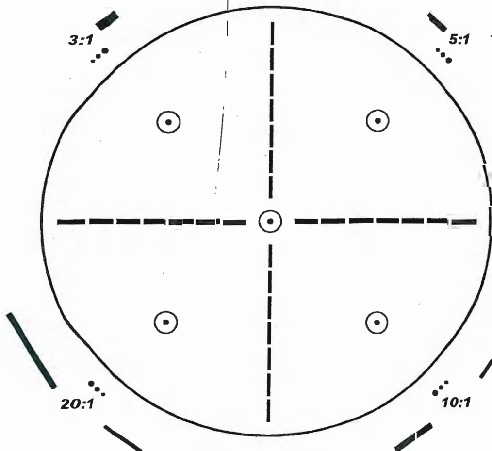
FIG. A1.1 Design of RIB Eye-piece Graticule
