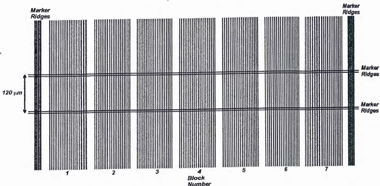
FIG. A2.1 HSE/NPL Phase Test Slide
