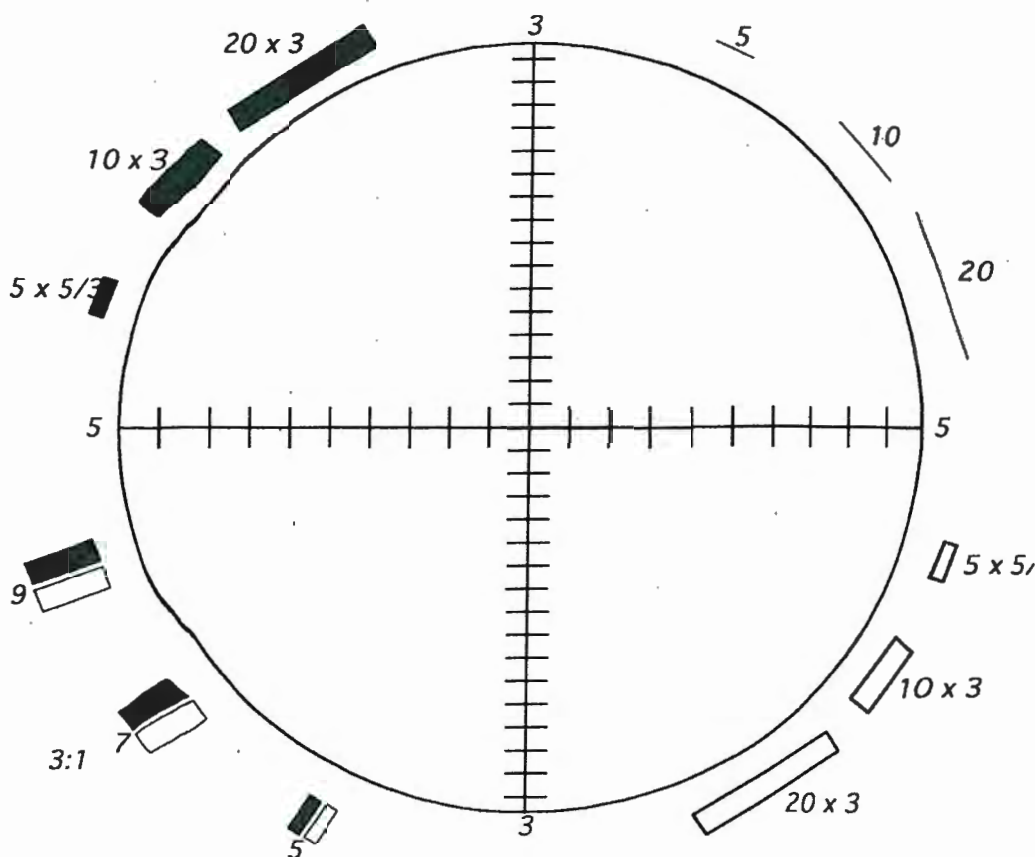
FIG. A1.2 Design of Walton-Beckett Eyepiece Graticule
