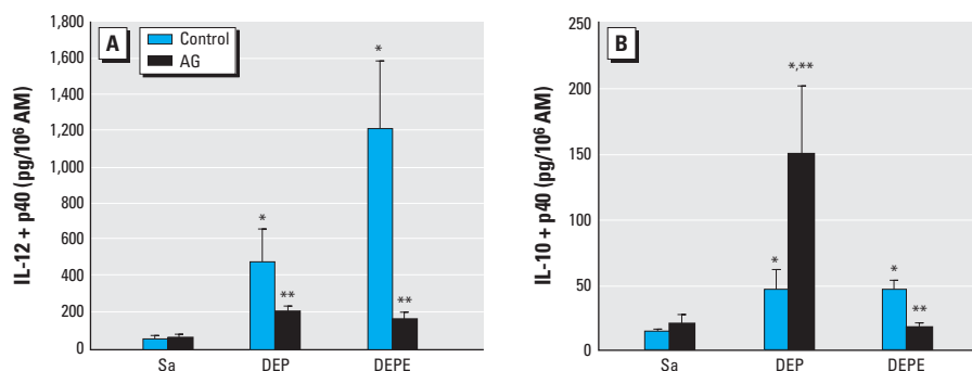
Figure 3. Role of NO in DEP- and DEPE-mediated pro- and antiinflammatory cytokine production by AM. Sa, saline. AM cells were isolated from different exposure groups with or without AG treatment. IL-12 (A) and IL-10 (B) production in the supernatant of the AM culture medium, at 37°C for 24 hr, was assayed using ELISA kits ( n = 6-8 ).
