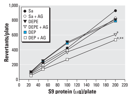
Figure 5. Effects of AG treatment on lung S9-dependent 2-AA mutagenicity in S. typhimurium strain YG1024. Sa, saline. Lung S9 were isolated at 1 day after saline, DEP, or DEPE exposure with or without AG treatment. For each sample, Ames assays were performed on duplicate plates. The spontaneous revertants ( 29 \pm 4 /plate) were subtracted from the number of revertants obtained for each assay. Results are presented as mean \pm SE ( n = 3 ).
