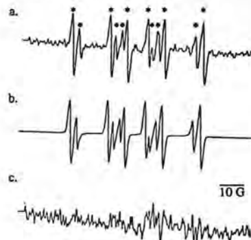
FIGURE 3. EPR spectrum of the photolysis (3 min) reaction mixture of a partially degassed solution of \text{CpW(CO)}_3\text{CH}_3 (1, 0.3 mM) and DMPO (20 mM) in 10% DMSO/tris buffer (10 mM, pH 8) at ambient temperature with a medium-pressure mercury lamp: (a) experimental spectrum; (b) simulated spectrum; and (c) difference spectrum (experimental – simulated spectra). All spectra are plotted on the same vertical scale, and the parameters for the experimental spectrum are the following: gain = 2.5 \times 10^4 , frequency = 9.434 GHz, power = 50 mW, modulation amplitude = 2 G, modulation frequency = 100 kHz, time constant = 0.250 ms, sweep width = 160 G, sweep time = 240 s. Hyperfine coupling constants obtained by simulation are reported in the text. Peaks marked by * result from \text{DMPO-CH}_3 and those marked by \blacklozenge are assigned to \text{DMPO-CO}_2^- .
