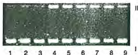
FIGURE 1. Photoinduced cleavage of pBR322 DNA (30 \mu\text{M}/\text{bp} in 10% DMSO/10 mM Tris buffer, pH 8) by \text{CpW(CO)}_3\text{CH}_3 (1): lane 1, DNA alone; lane 2, DNA alone, irradiated; lane 3, DNA + complex (720 \mu\text{M} ), no irradiation; lanes 4 through 9, DNA + complex (720, 360, 180, 90, 45, and 23 \mu\text{M} , respectively). Reactions in lanes 4–9 were irradiated with Pyrex-filtered light from a 450-W medium-pressure mercury arc lamp for 20 min.
