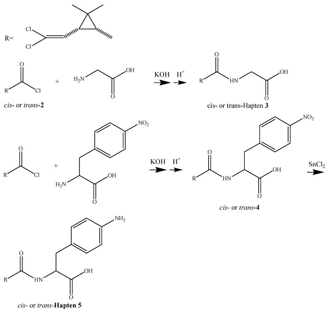
Figure 2. Scheme for the synthesis of the target analyte ( cis/trans -DCCA-glycine, hapten 3) and cis/trans -hapten 5.
