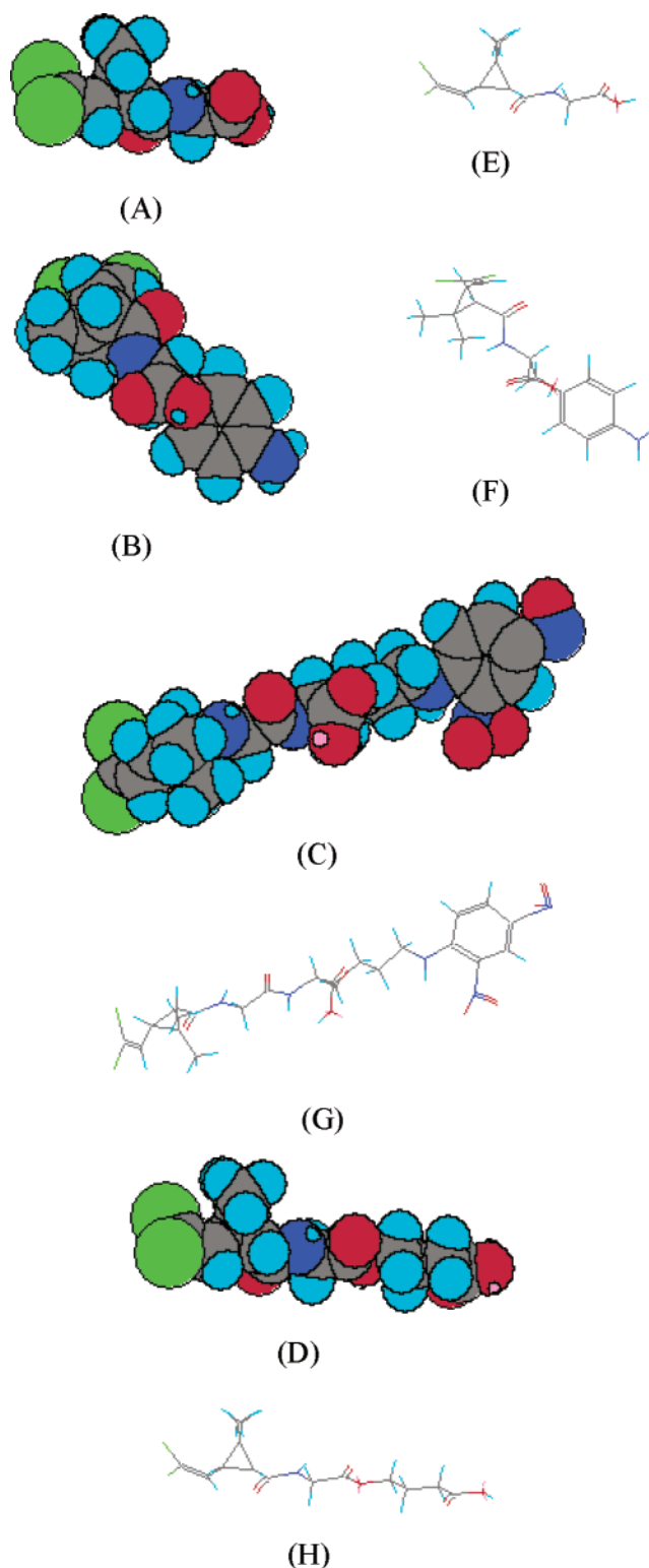
Figure 5. Optimized molecular model of (A,E) DCCA-glycine, (B,F) hapten 5, (C,G) hapten 9, and (D,H) hapten 24; A–D, space filling models, and E–H, stick models.
