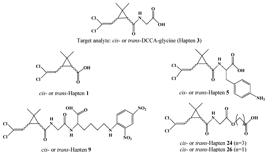
Figure 1. Target analyte and haptens designed.
