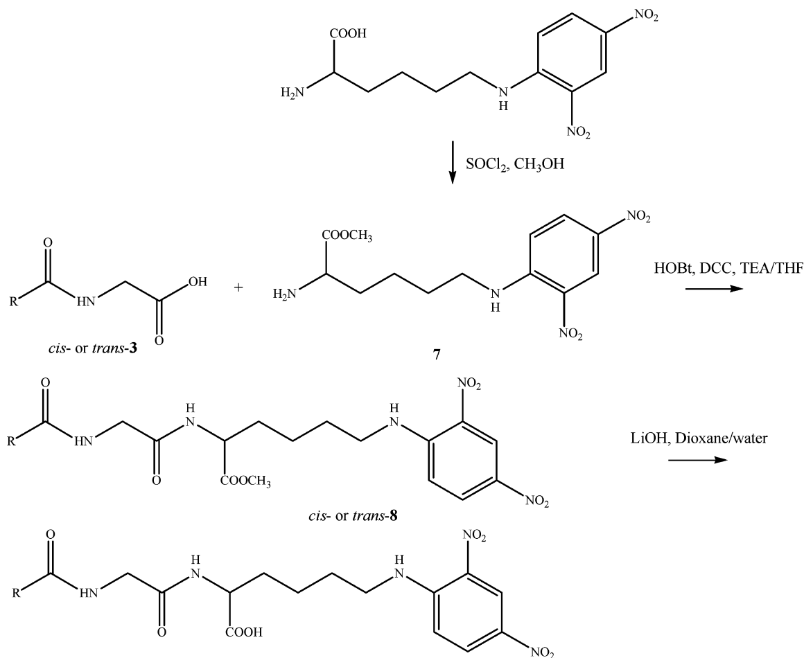
Figure 3. Scheme for the synthesis of cis/trans -hapten 9.
