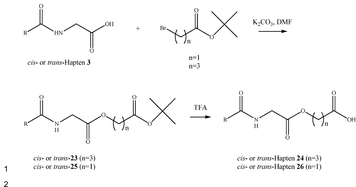
Figure 4. Scheme for the synthesis of cis/trans -haptens 24 and 26 .
