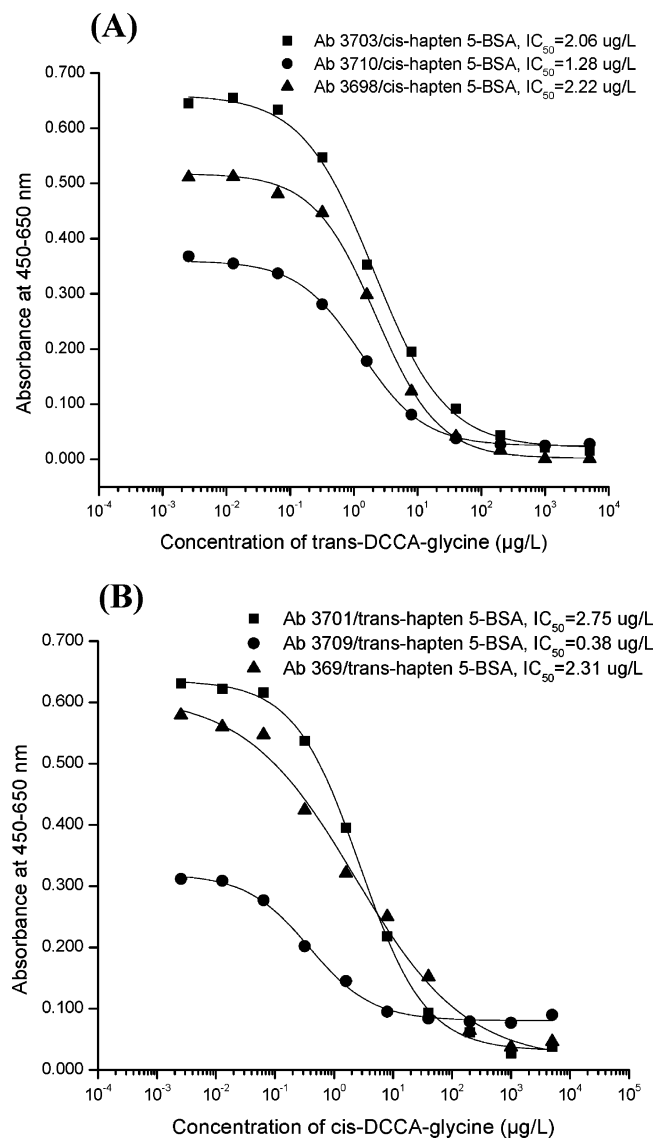
Figure 6. Six ELISA inhibition curves for trans -DCCA-glycine (A) and cis -DCCA-glycine (B) under unoptimized conditions. The reagent concentrations were as follows: the assay for trans -DCCA-glycine using Ab 3703, 1:32 000; Ab 3710, 1:8000; and Ab 3698, 1:16 000; and coating antigen cis -haptin 5–BSA, 1, 5, and 2 \mu g/mL, respectively. The assay for cis -DCCA-glycine using Ab 3701, 1:16 000; Ab 3709, 1:8000; and Ab 369, 1:16 000; and coating antigen trans -haptin 5–BSA, 1 \mu g/mL. The dilution ratios of the Ab are the final concentrations in the wells.
